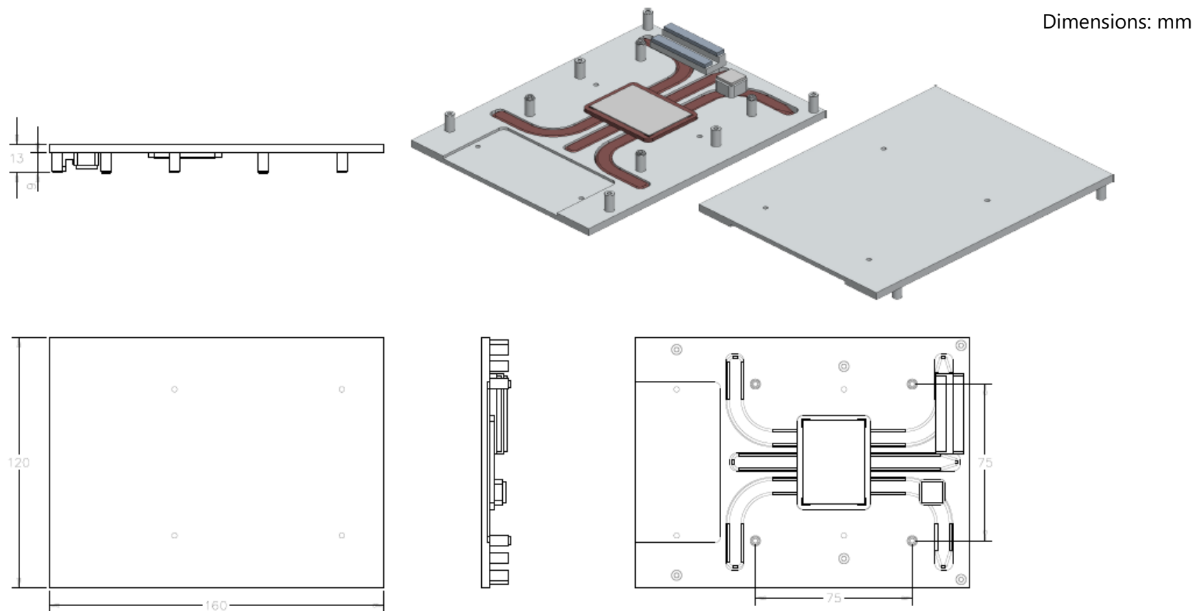
Figure 6 – Heatspreader: HTS
