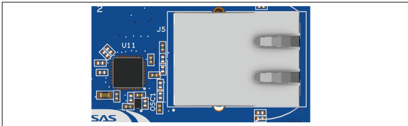
Figure 16. Ethernet Connector
