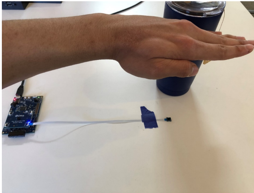
Figure 10. STR Setup
