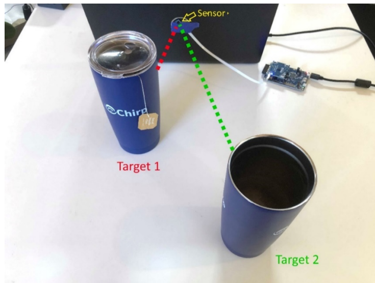
Figure 8. Two-Target setup
