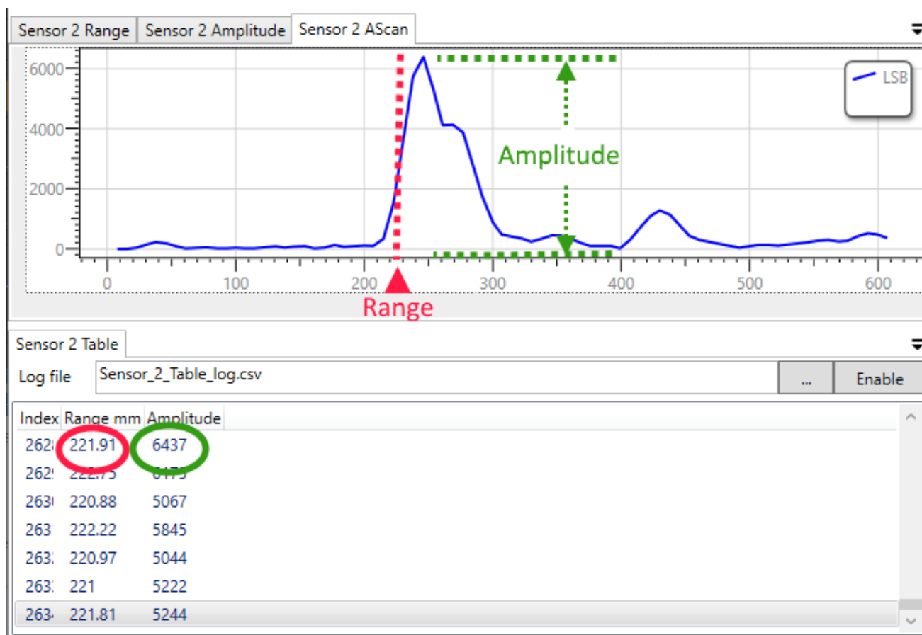
Figure 7. Single-Target A-Scan
