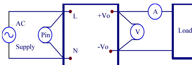
Figure 1. CFM300M Series Test Setup
