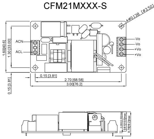
Figure 3. CFM21M series Mechanical Outline Diagram
