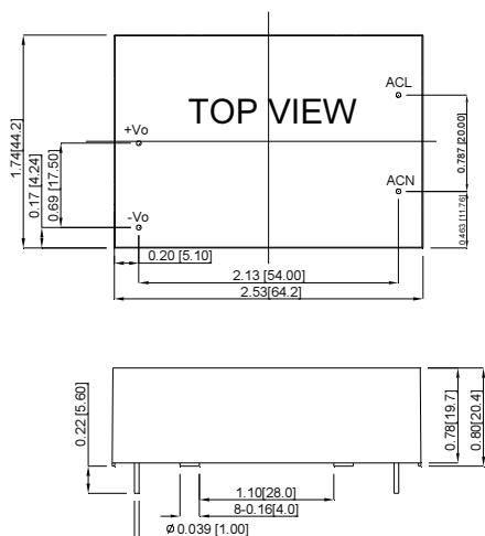
Figure 3. CFM21M series Mechanical Outline Diagram
