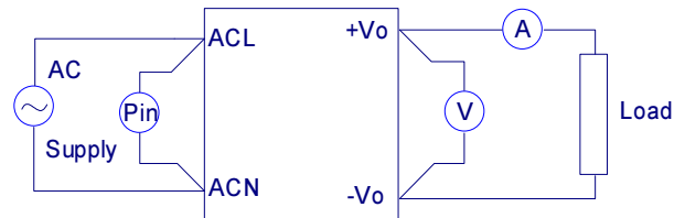
Figure 1. CFM20S Series Test Setup
