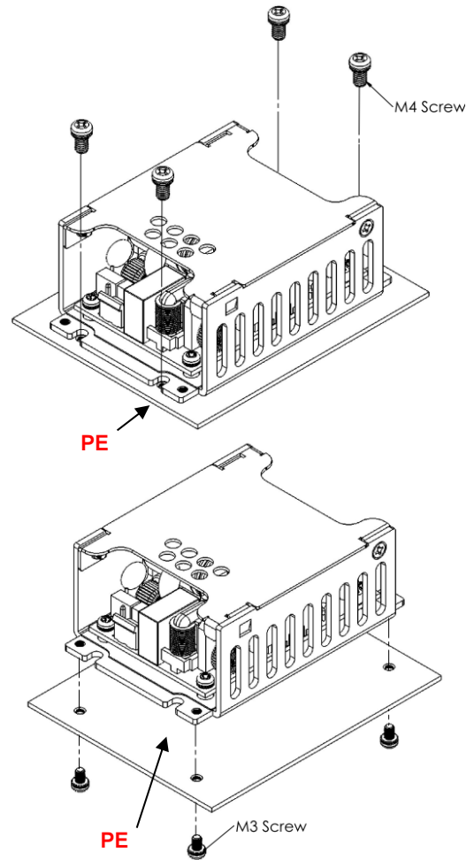
CFM130SXXX-C installation diagram
