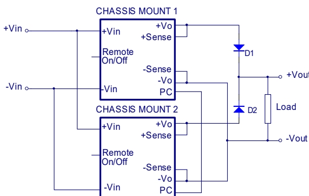
Simple Redundant Operation Connect Circuit
