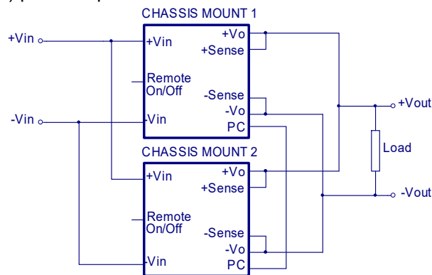
Simple Parallel Operation Connect Circuit
