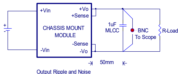
Output Ripple and Noise
