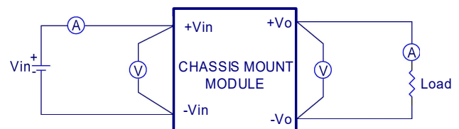
CFB750-300SXX-CMFD Series Test Setup
