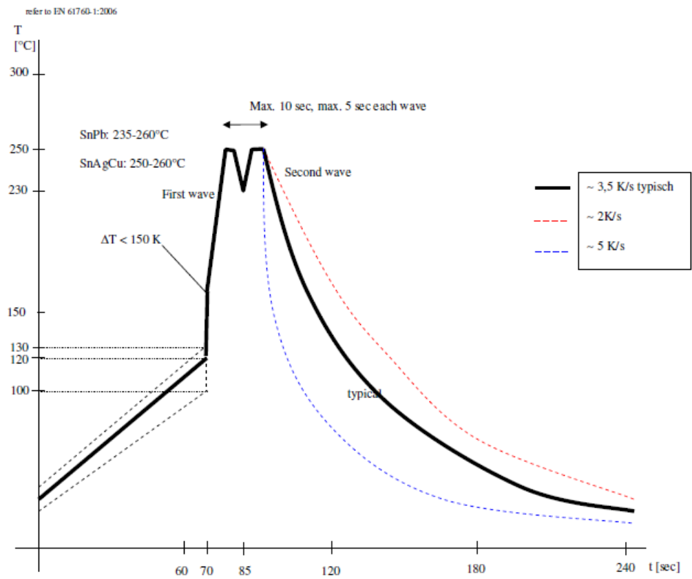
Figure 32. Classification wave soldering profile for THT components
