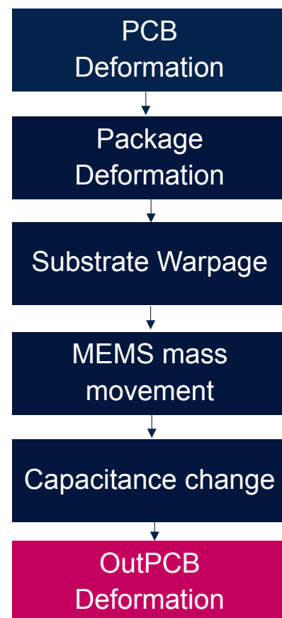
Figure 21. Consequences of thermomechanical stress
