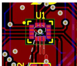
Figure 15. Examples of top side placement
