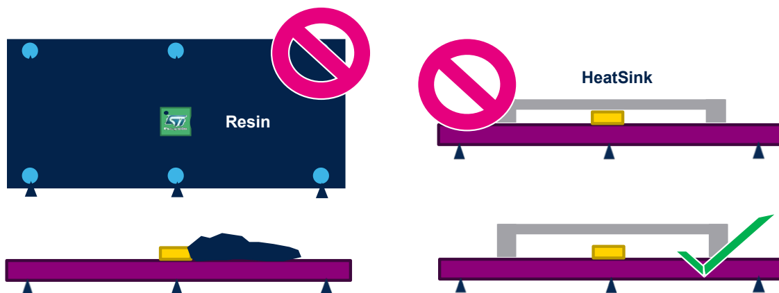
Figure 25. Examples of sources of stress to the sensor
