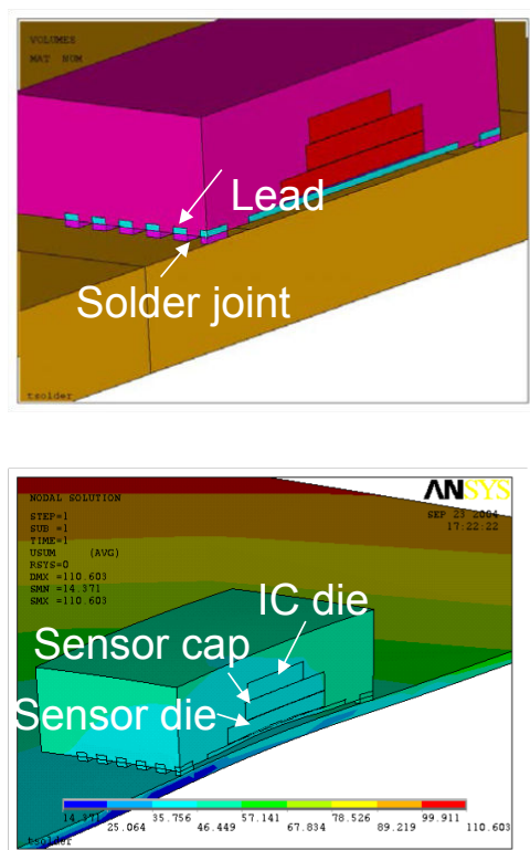
Figure 21. Consequences of thermomechanical stress
