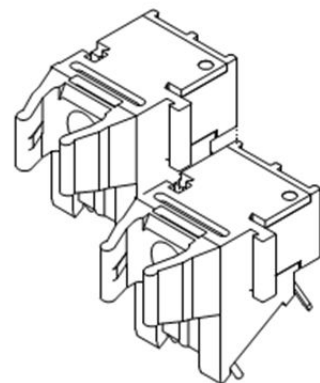
Figure11. Interlocked (stacked) horizontal, vertical and tilted (30°) packages
