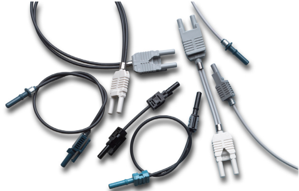
Figure 28. Simplex and duplex POF cable with crimp ring and crimpless solutions
