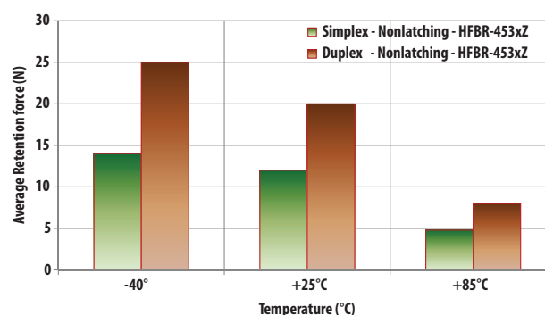
Figure 17a. Average Retention force of simplex and duplex connectors over industrial temperature range
