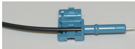
Figure 23. POF cable termination using simplex crimpleless connector
