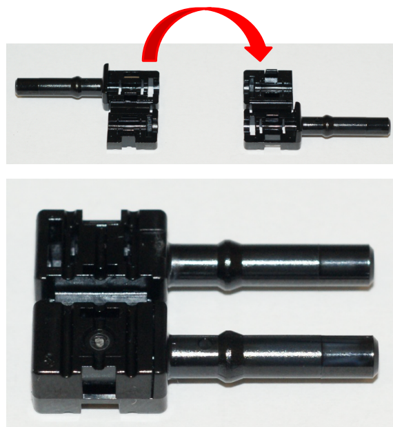
Figure17. Crimpless Duplex Connector
