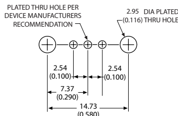
Recommended hole pattern for 8223-CL03G
