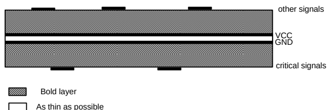
Figure 23. Right: VCC and GND planes are close together
