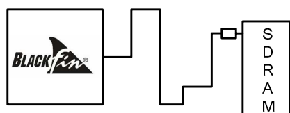
Figure 20. Wrong: Trace edges lack rounding
