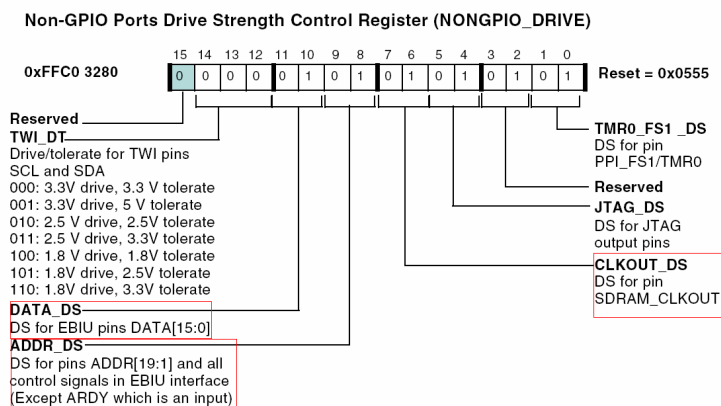
Figure 32. The Drive Strength control register of the BF52x
