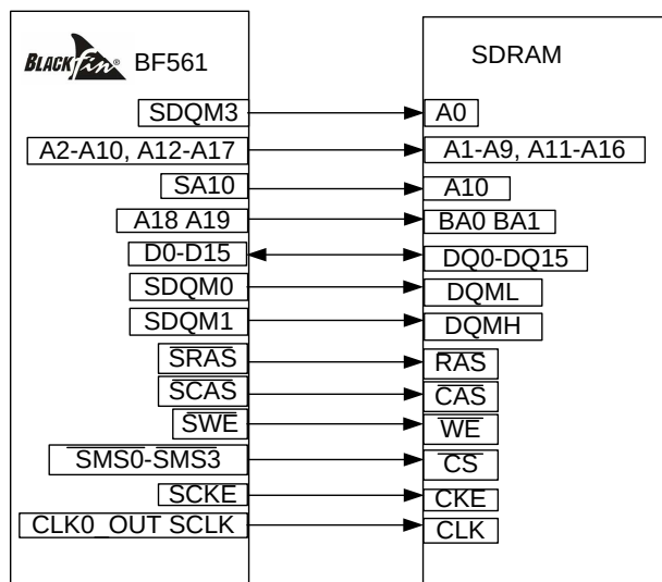
Figure 14. ADSP-BF561 processors: connections between the Blackfin processor and 16-bit SDRAM
