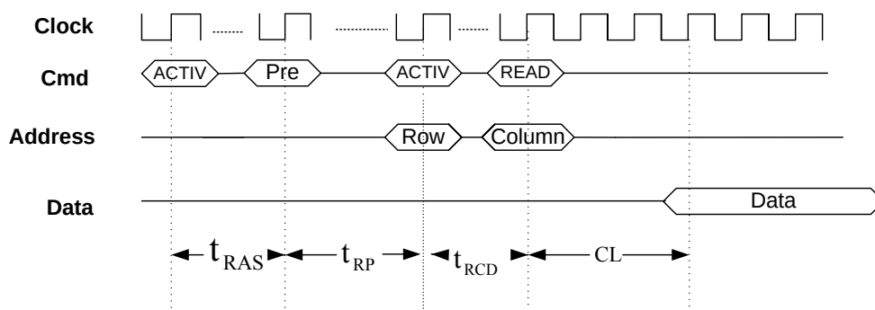
Figure 2. SDRAM Timing
