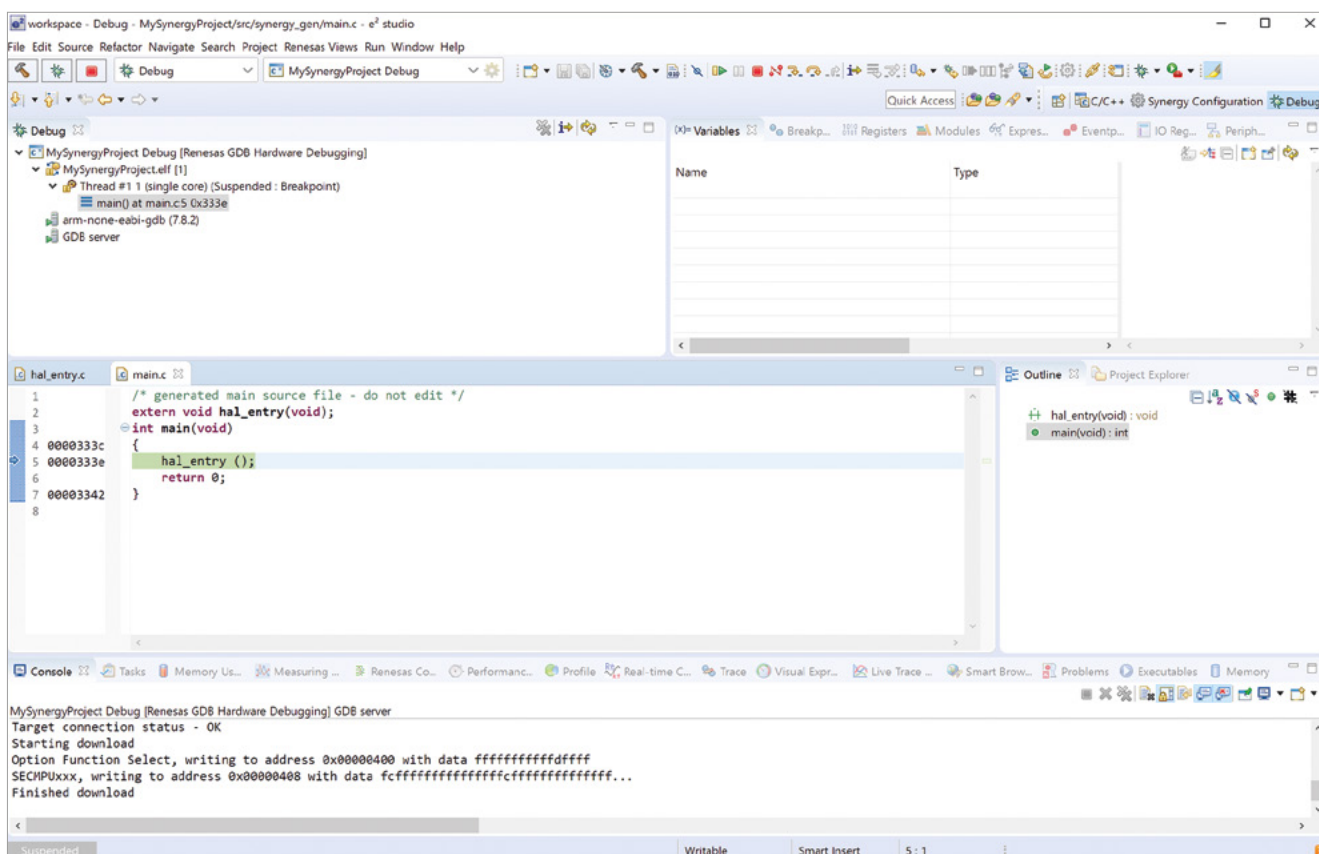
Figure 7-4: The debug perspective of e 2 studio
