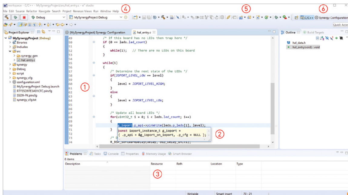
Figure 5-1: The workbench of e² studio consisting of editors (1), Smart Manuals (2), views (3), menu bar (4), tool bars (5) and perspectives (6)
