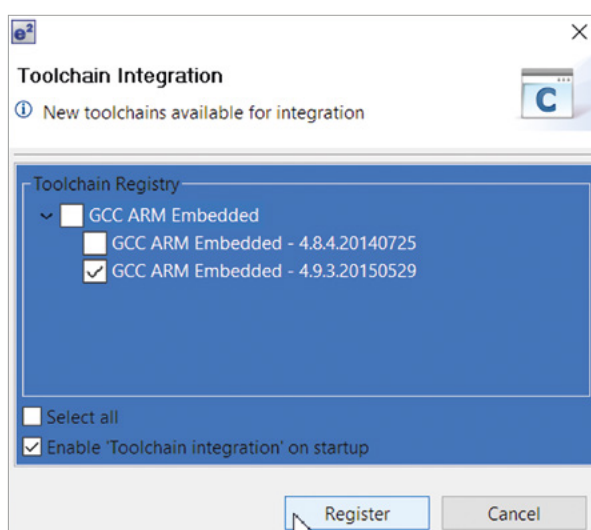
Figure 4-9: Failing to select the installed tool chain here will result in build problems
