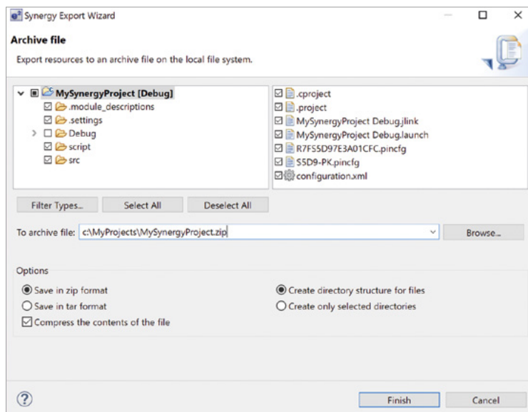
Figure 5-5: The Export Wizard in e 2 studio
