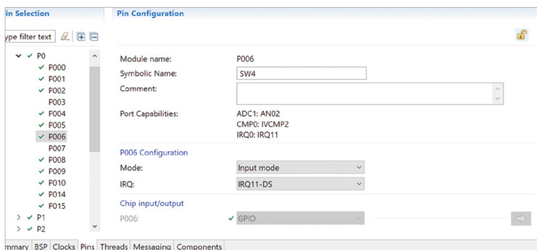
Figure 9-6: Port P006 needs to be configured as input to IRQ11
