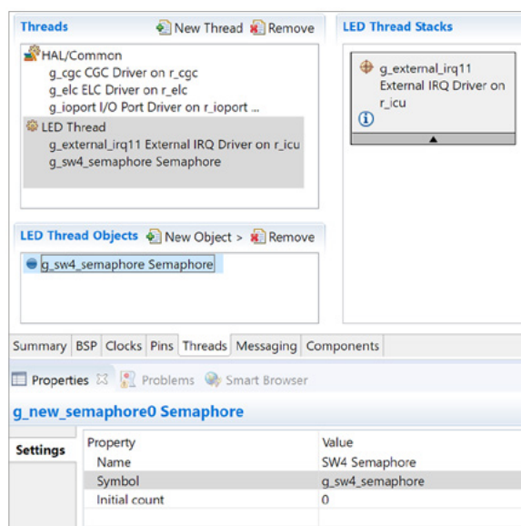
Figure 9-5: This is what the Threads tab should look like after the LED Thread and the semaphore has been added
