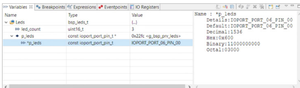
Figure 8-9: Variables and their values can be observed in the variables tab
