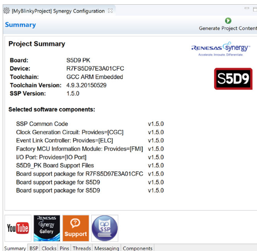
Figure 8-6: The summary tab of the Synergy Configurator
