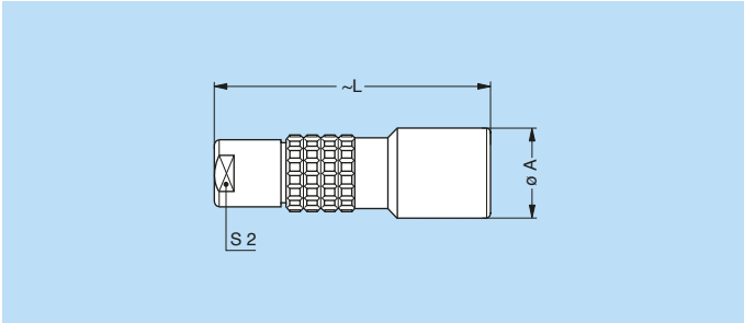
Cable collet and nut for fitting a bend relief 1)
