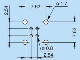
P11 - EPG-EXG (0B/1B.306) Screw mount
