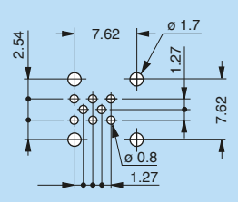
P11 - EPG-EXG (1B.310) Screw mount
