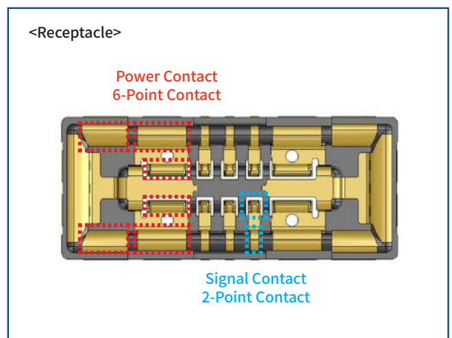
Multi-point Contact
