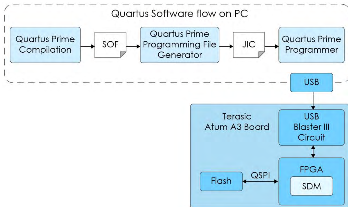
Figure 5-1 Programming Flow
