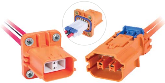
2 Way 180° Connection System with Pluggable Inner Connector
