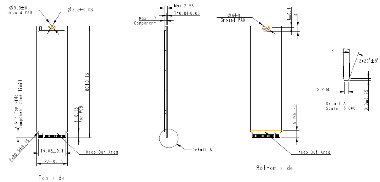
Figure 10-1 Physical Dimensions
