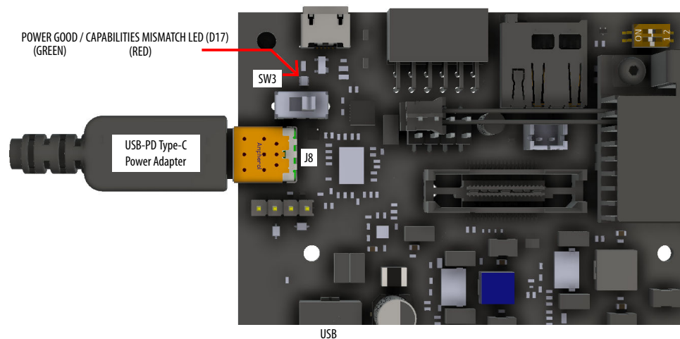
Figure 7. Powering the Agilex 3 FPGA and SoC C-Series Development Board
