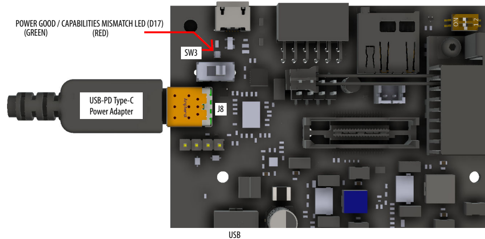
Figure 31. Powering the Agilex 3 FPGA and SoC C-Series Development Board
