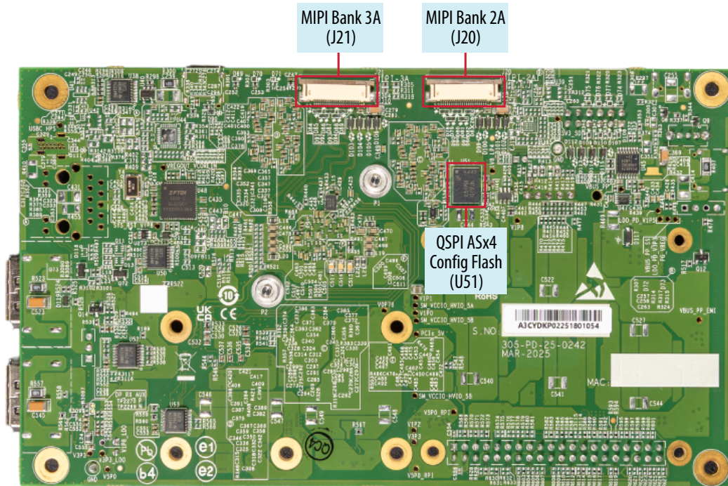
Figure 28. Components in Agilex 3 FPGA and SoC C-Series Development Kit (Bottom View)
