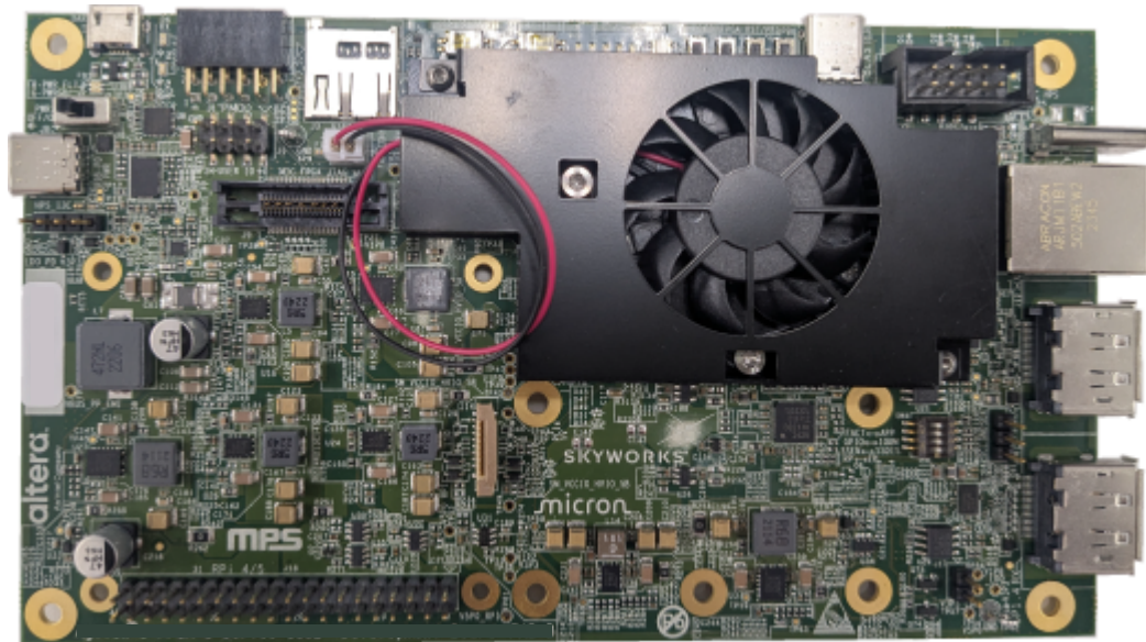
Figure 3. Agilex 3 FPGA and SoC C-Series Development Kit (Top View)
