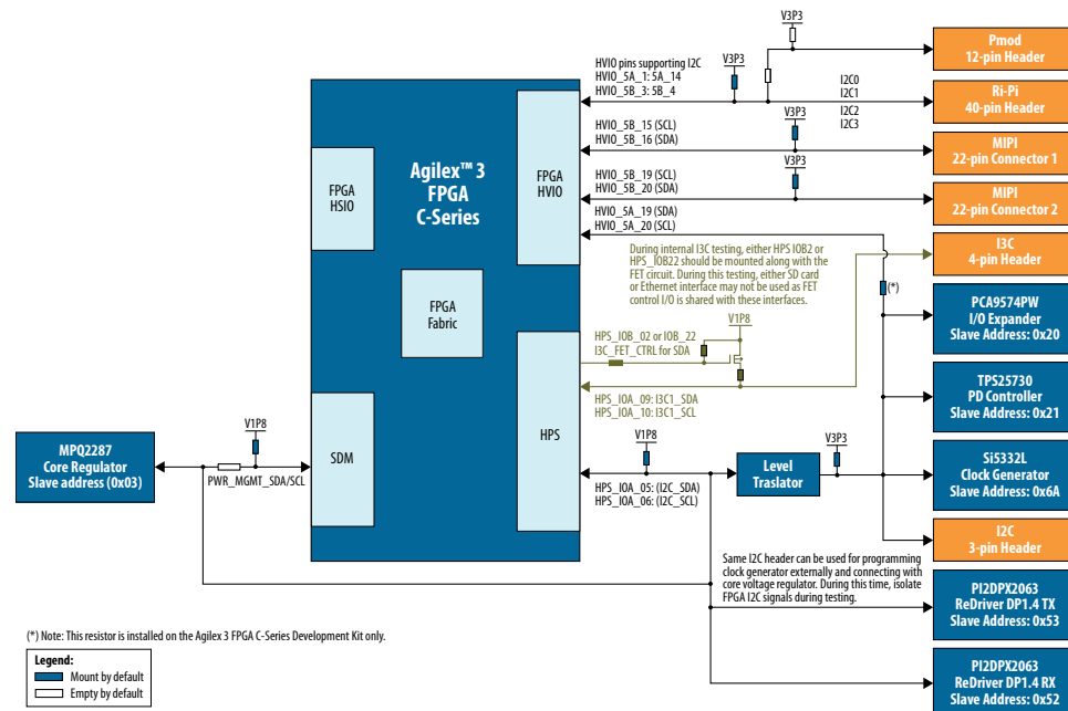
Figure 29. I 2 C Block Diagram
