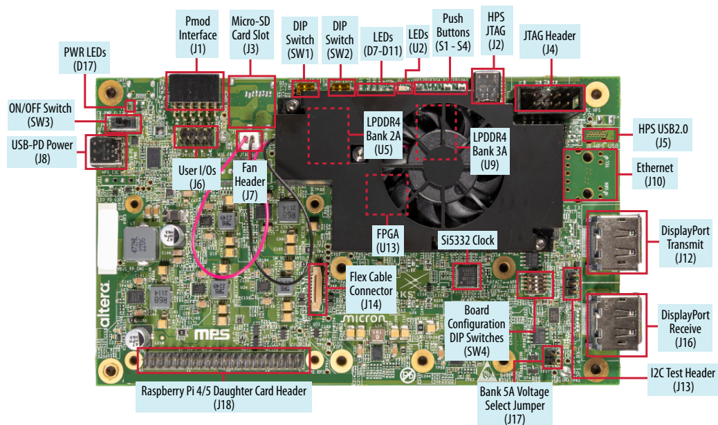
Figure 27. Components in Agilex 3 FPGA and SoC C-Series Development Kit (Top View)
