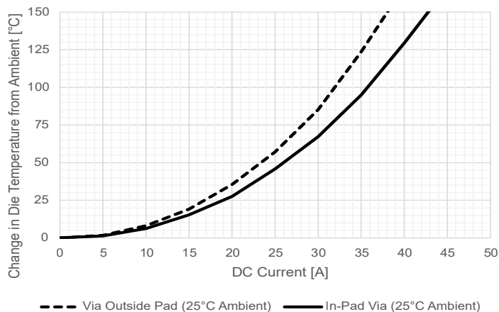
Figure 9: Comparison of Die-Temperature Increase With and Without In-Pad Vias at T_A = 25^\circ\text{C}
