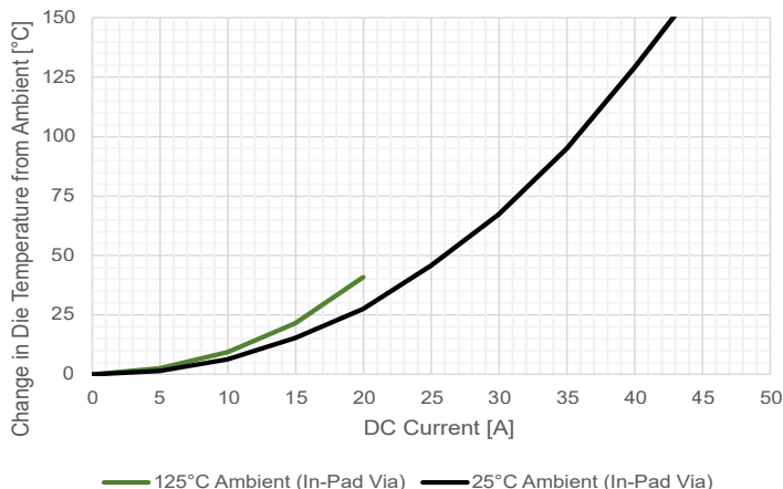
Figure 10: Comparison of Die-Temperature Increase at T_A = 25^\circ\text{C} and T_A = 125^\circ\text{C} With In-Pad Vias
