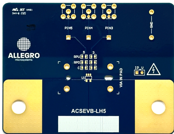
Figure 11: LH Package Allegro Evaluation Board
