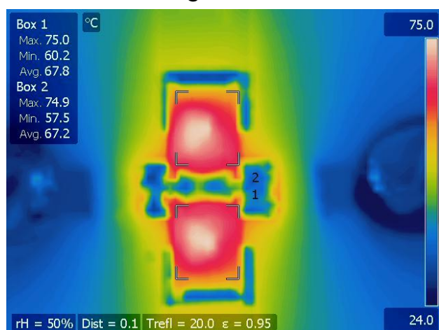
Figure 3: Resistor Power Handling Equivalent Heating
