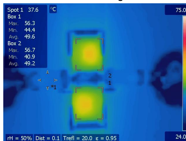
Figure 2: Resistor Power Handling – \frac{1}{2} Watt
