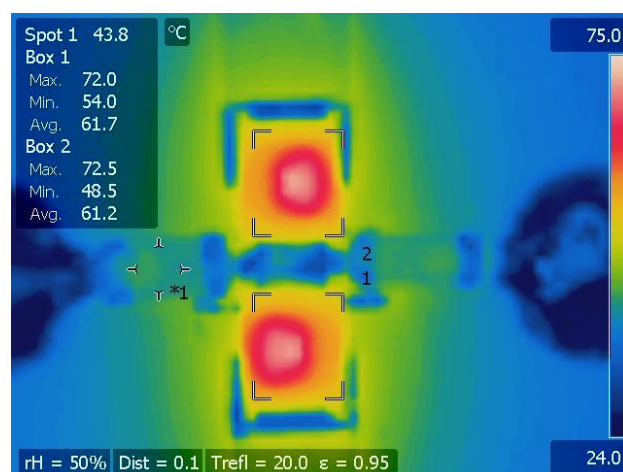
Figure 3: Resistor Power Handling Equivalent Heating
