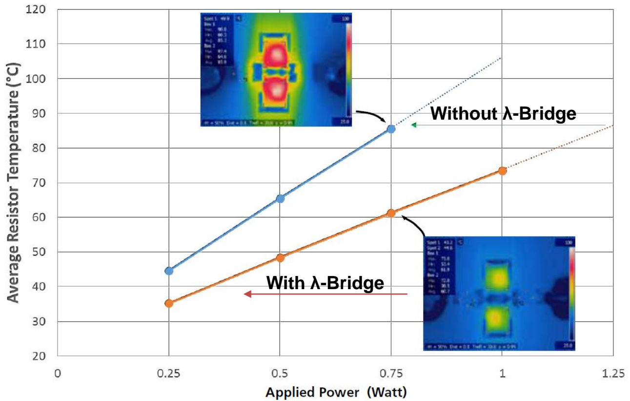
Figure 4: \lambda -Bridge Test Results
