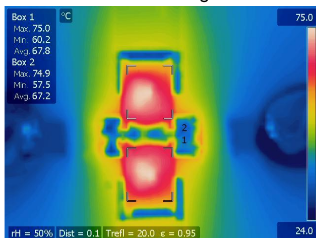
Figure 2: Resistor Power Handling – \frac{1}{2} Watt
