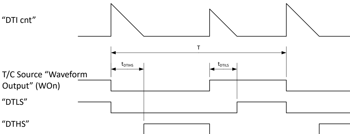
Figure 24-5. Dead-Time Generator Timing Diagram
