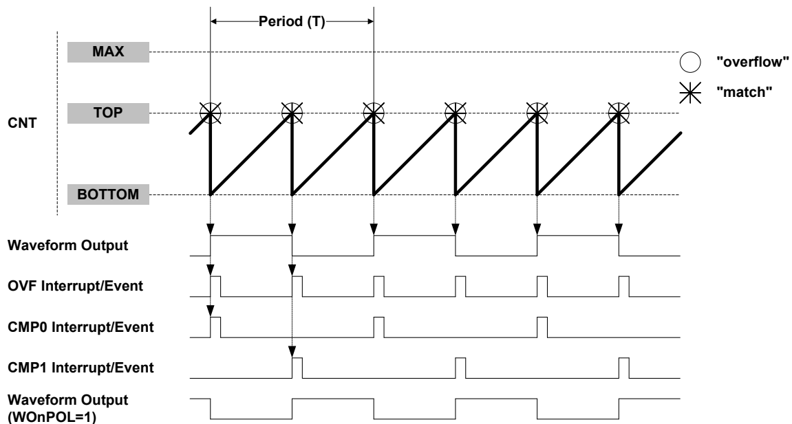
Figure 25-4. Frequency Waveform Generation
