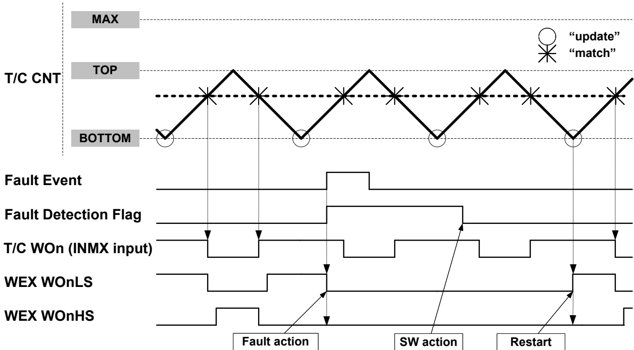
Figure 24-9. Cycle-By-Cycle Mode Fault Handling
