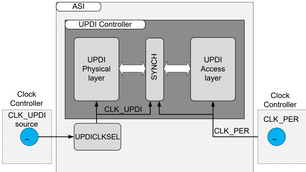
Figure 34-3. UPDI Clock Domains
