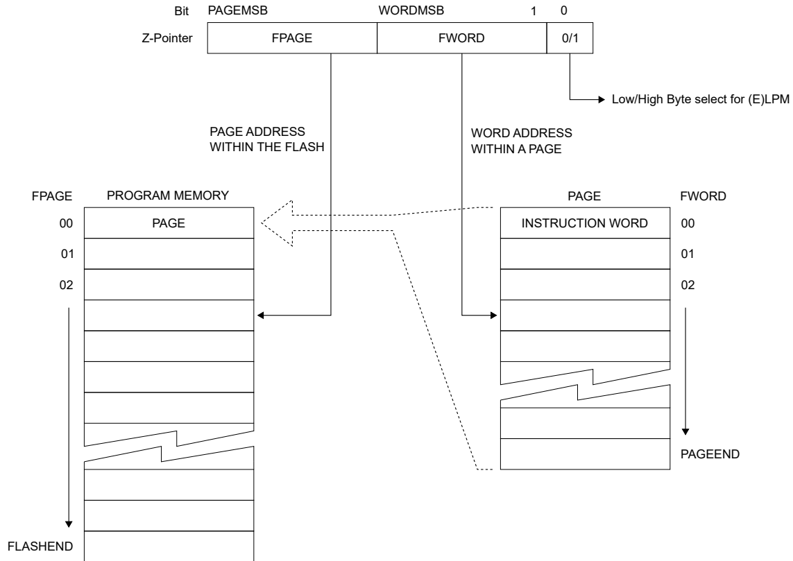
Figure 11-4. Flash Addressing for Self-Programming
