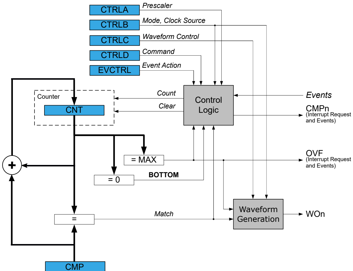
Figure 25-1. Timer/Counter Type F Block Diagram
