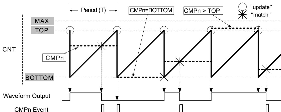
Figure 25-7. 8-Bit PWM Mode
