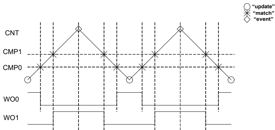
Figure 24-3. PWM Generation for CWCMB
