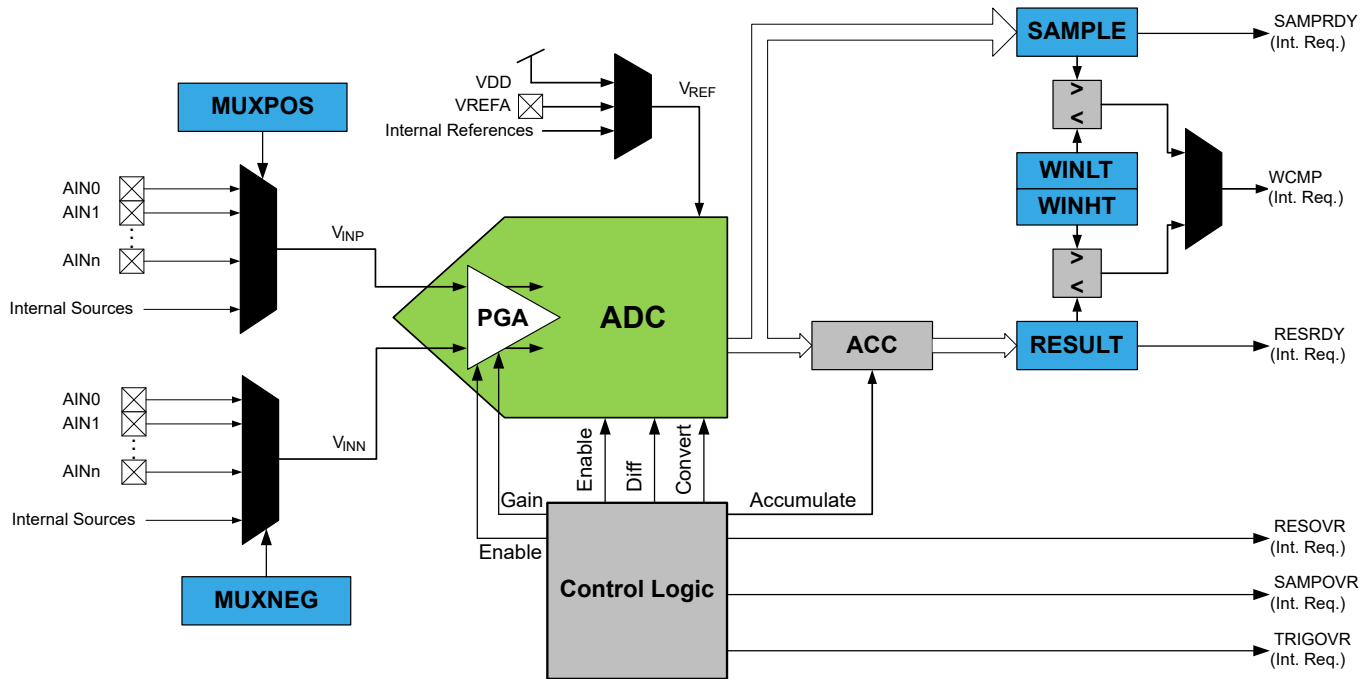
Figure 33-1. Block Diagram
