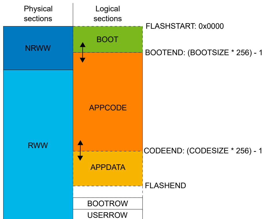
Figure 11-2. AVR EB Family Flash Sections
