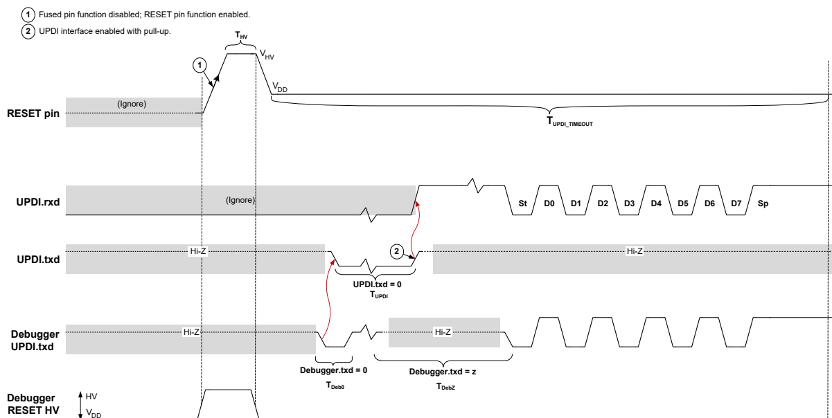
Figure 34-6. UPDI Enable Sequence by High-Voltage (HV) Programming
