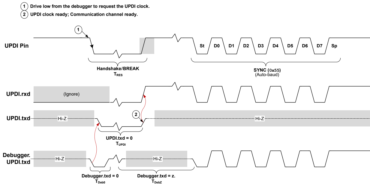
Figure 34-5. UPDI Enable Sequence
