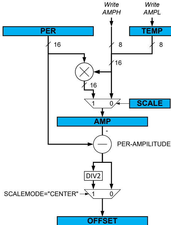
Figure 23-15. Write to Amplitude and Offset Registers
