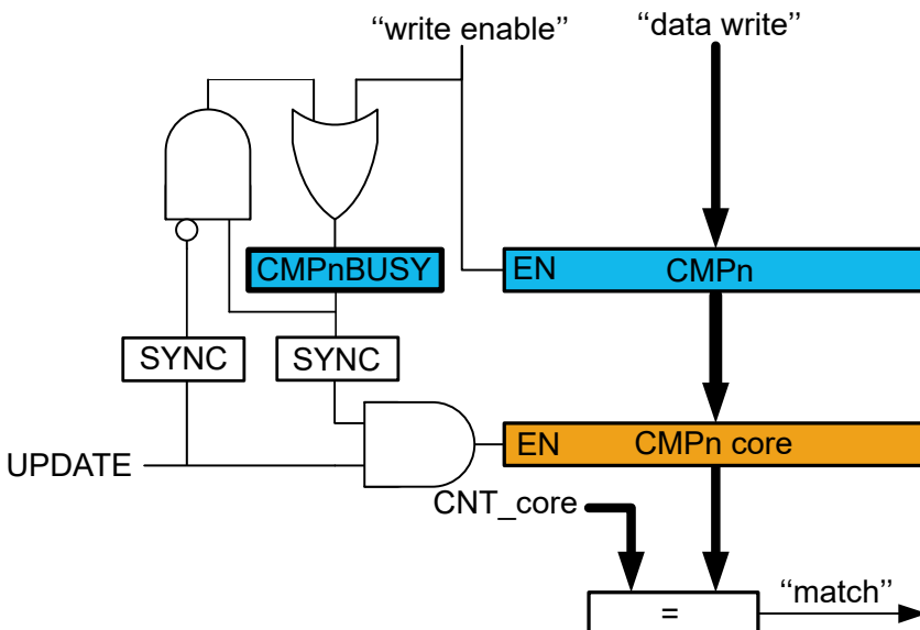
Figure 25-3. Double Buffering
