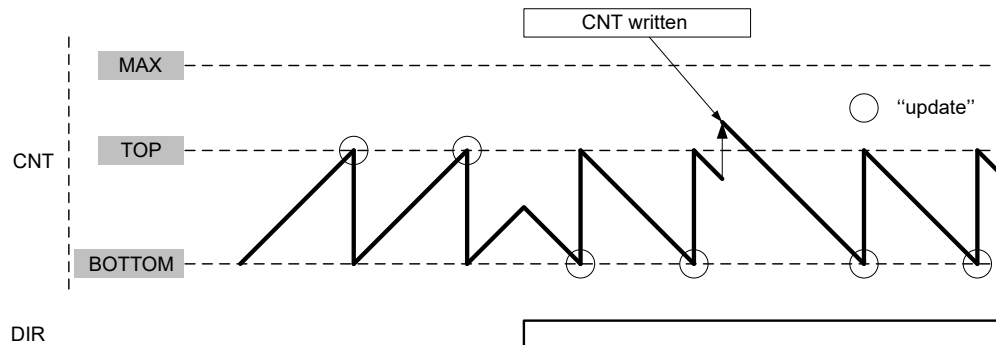
Figure 23-3. Normal Operation
