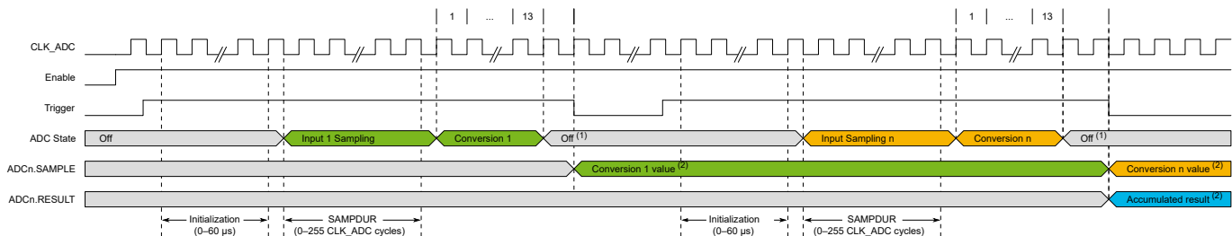
Figure 33-4. Timing Diagram - Series Accumulation
