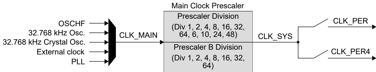
Figure 12-2. Main Clock and Prescaler
