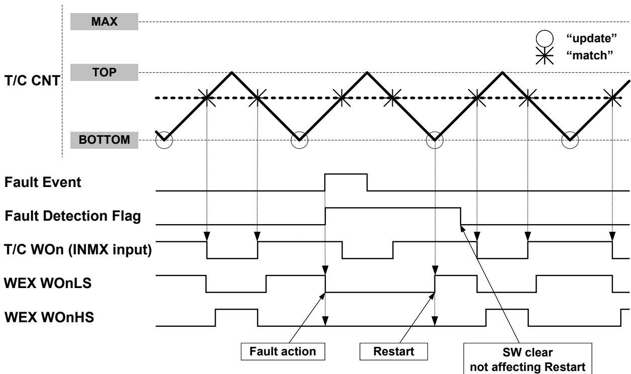
Figure 24-9. Cycle-By-Cycle Mode Fault Handling
