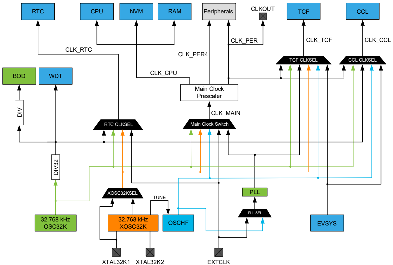
Figure 12-1. CLKCTRL Block Diagram
