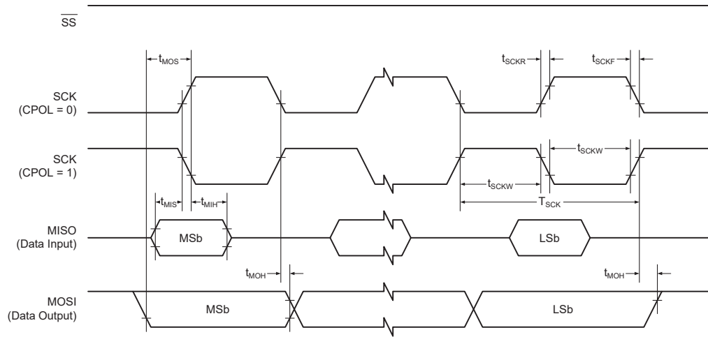
Figure 36-4. SPI - Timing Requirements in Host Mode
