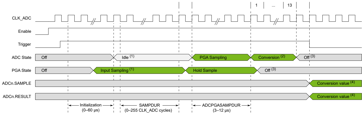
Figure 33-6. Timing Diagram - Single Conversion with PGA
