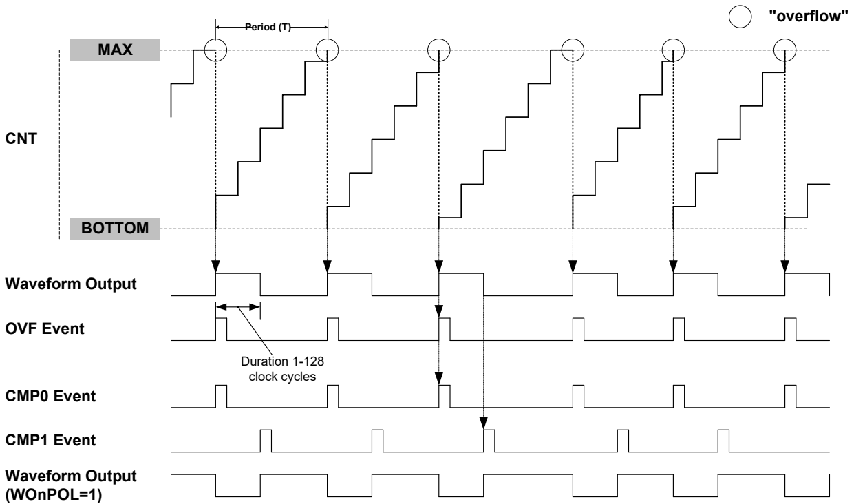
Figure 25-5. NCO Pulse-Frequency Waveform Generation
