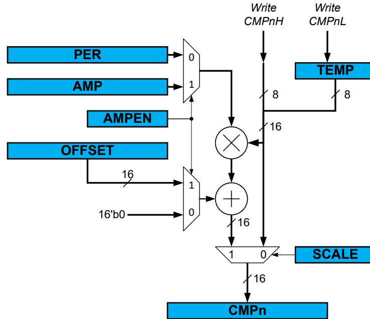
Figure 23-16. Writing Fractional Value to Compare Register
