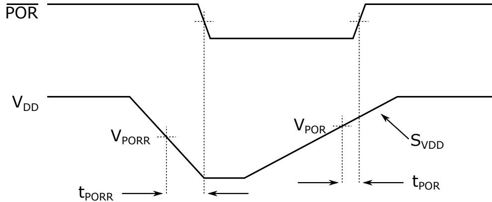
Figure 36-1. \overline{\text{POR}} and \overline{\text{POR}} Re-Arm with Slow Rising V_{\text{DD}}
