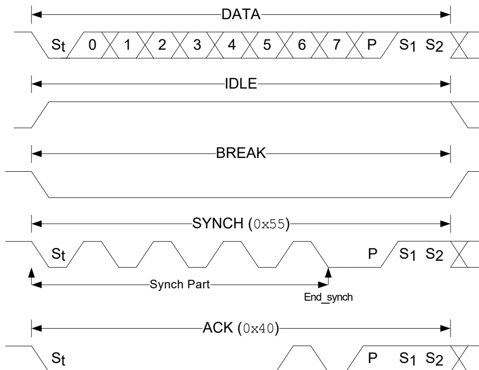
Figure 34-4. Supported UPDI Frame Formats
