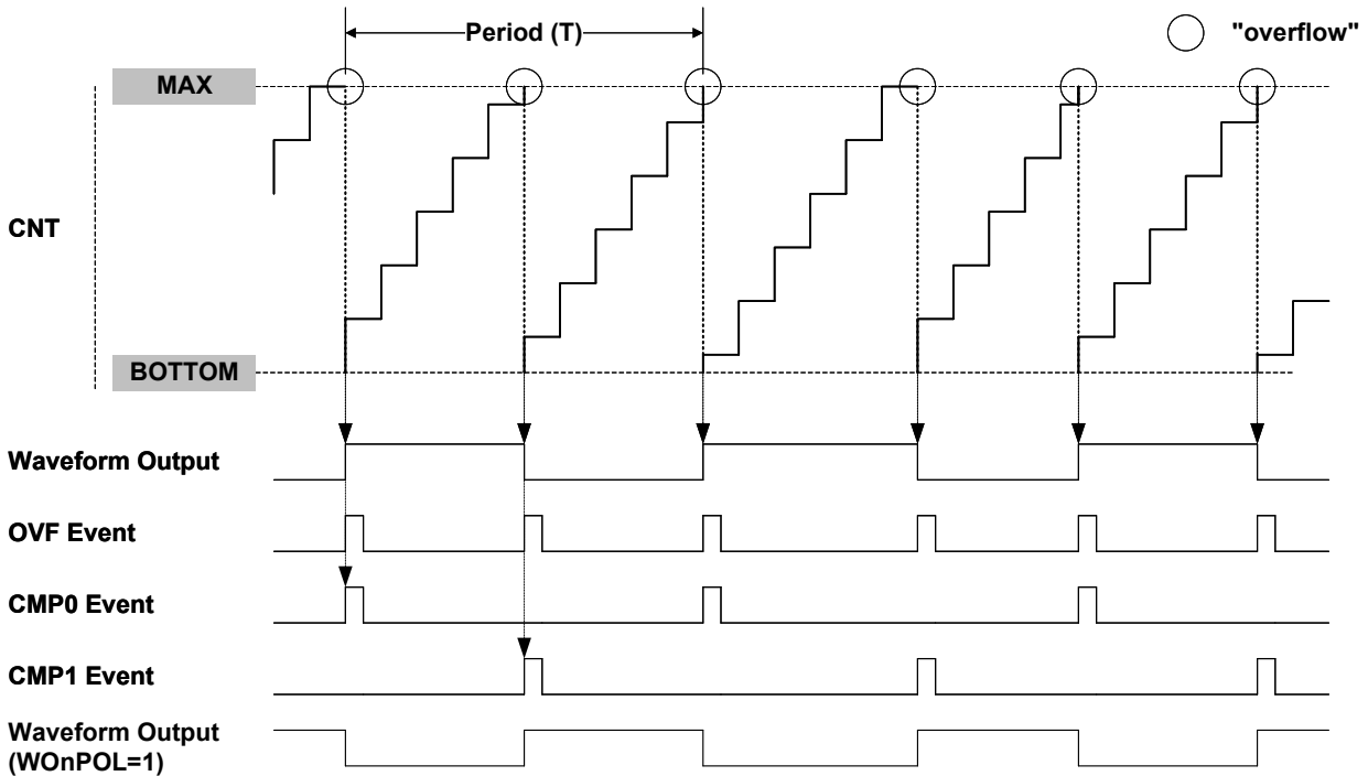
Figure 25-6. NCO Fixed Duty-Cycle Frequency Waveform Generation
