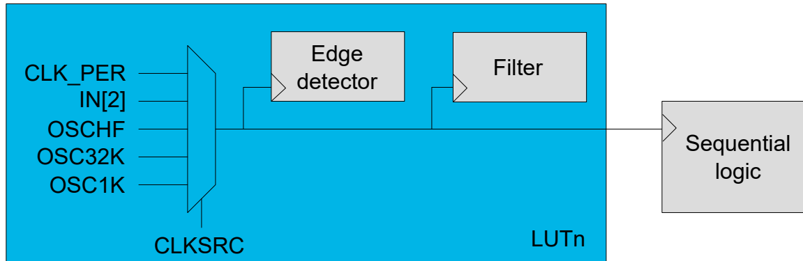
Figure 31-11. CCL Clock Sources
