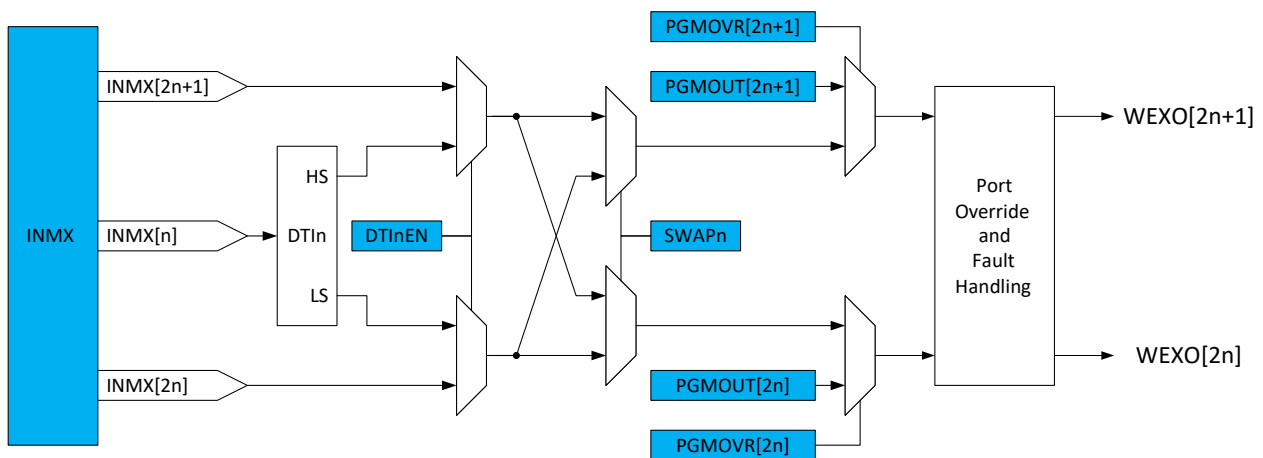
Figure 24-2. Waveform Extension Stage Details
