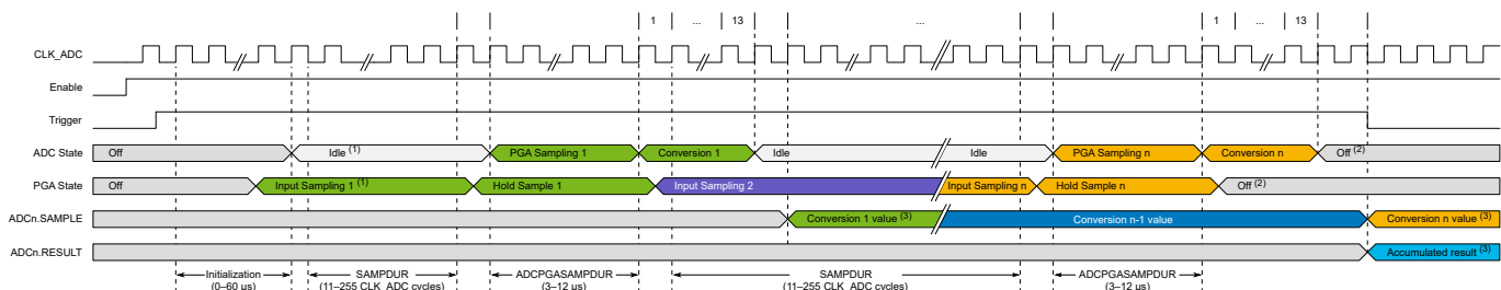
Figure 33-8. Timing Diagram - Burst Accumulation with PGA
