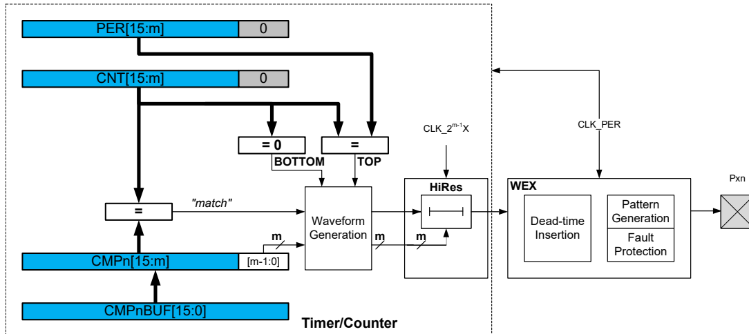
Figure 23-13. Timer/Counter with High-Resolution Extension
