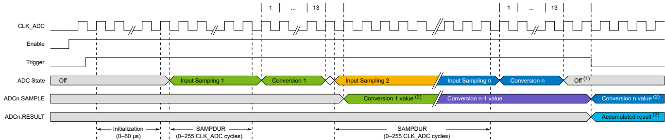
Figure 33-5. Timing Diagram - Burst Accumulation
