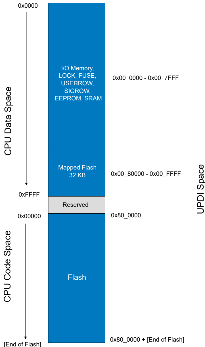
Figure 34-2. Memory Map, As Seen From The UPDI
