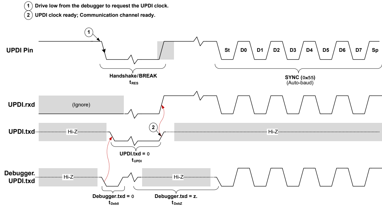
Figure 36-7. UPDI Enable Sequence with Dedicated UPDI Pin
