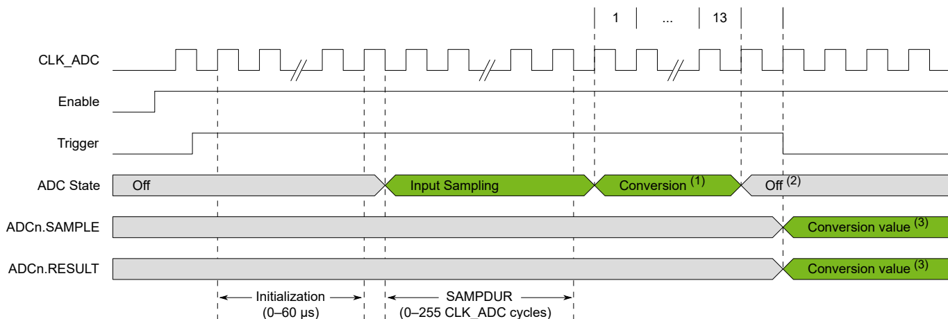
Figure 33-3. Timing Diagram - Single Conversion
