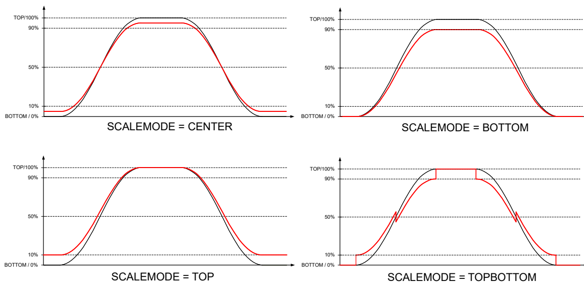
Figure 23-17. Scaled Writes (Amplitude = 90%)
