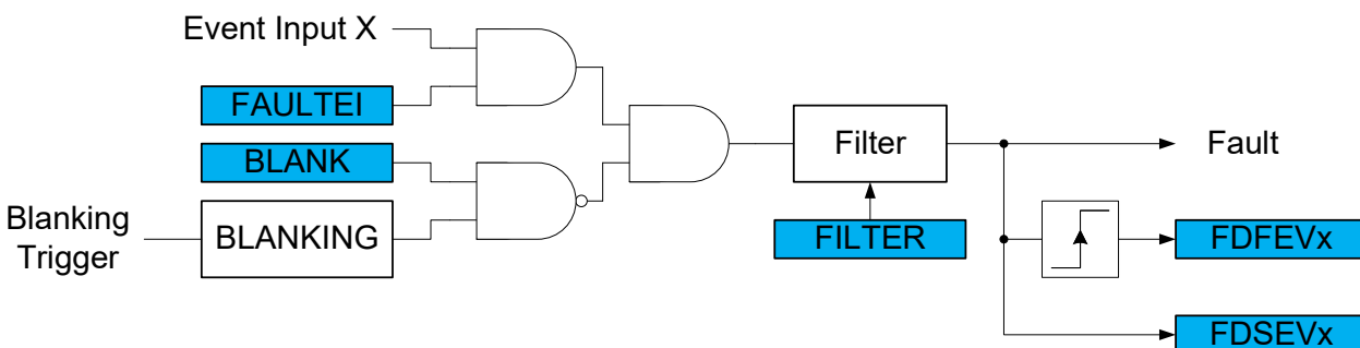
Figure 24-7. Filter and Blanking
