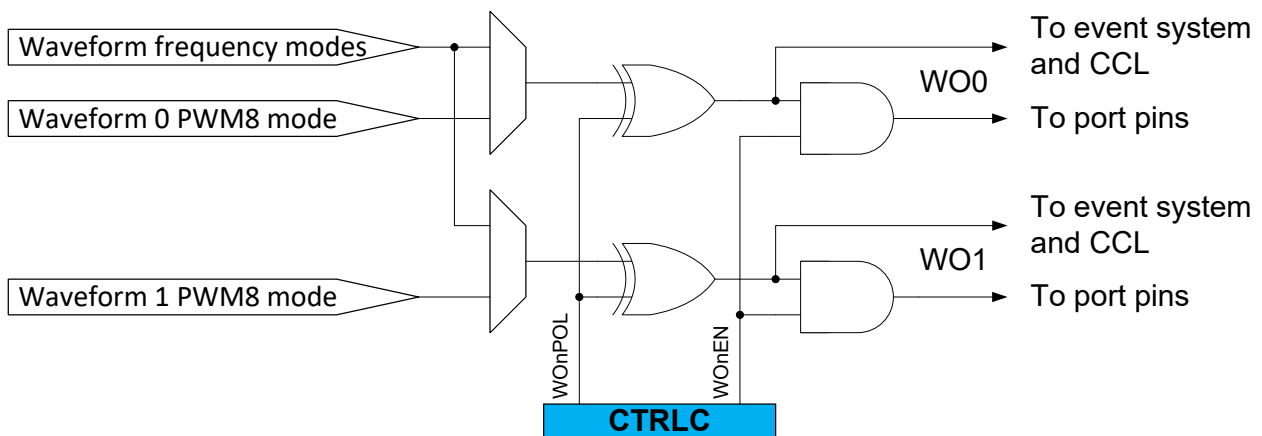
Figure 25-8. Waveform Output to the Pin, Event System and CCL
