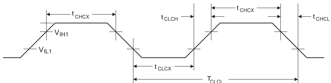
Figure 36-2. External Clock Waveform
