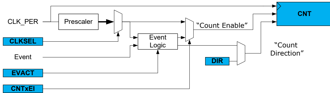
Figure 23-2. Timer/Counter Clock Logic
