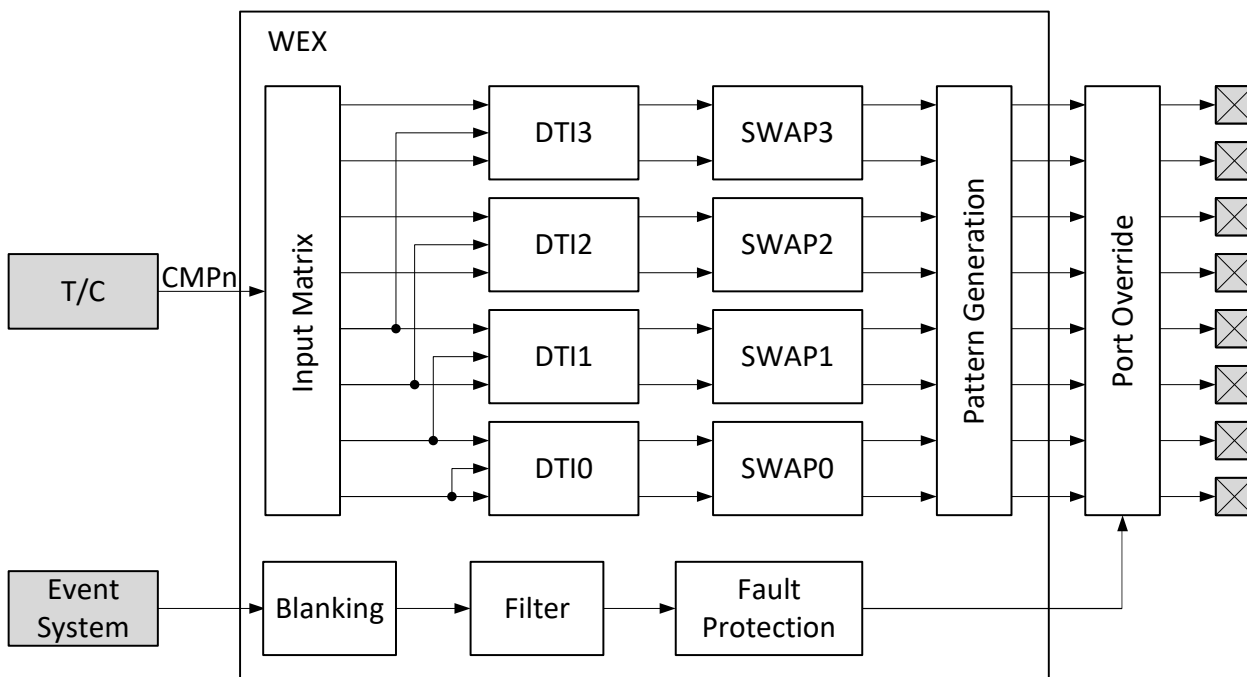
Figure 24-1. Block Diagram Overview
