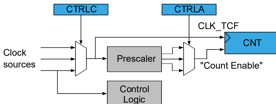
Figure 25-2. Timer/Counter Clock Logic
