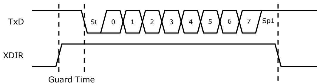
Figure 27-11. XDIR Drive Timing
