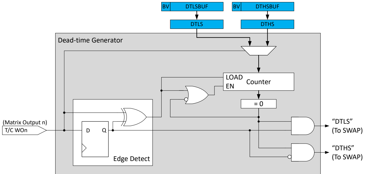
Figure 24-4. Dead-Time Generator Block Diagram
