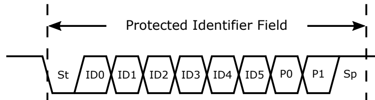
Figure 27-14. Protected Identifier Field and Mapping of Identifier and Parity Bits
