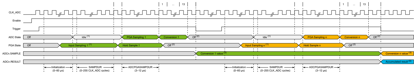
Figure 33-7. Timing Diagram - Series Accumulation with PGA
