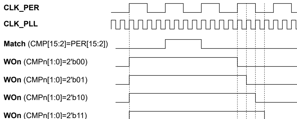
Figure 23-14. Duty Cycle Control
