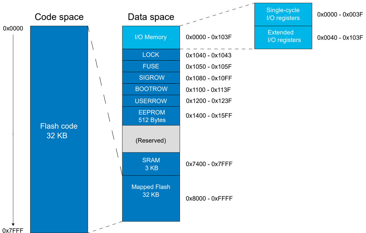
Figure 8-1. Memory Map: Flash 32 KB, Internal SRAM 3 KB, EEPROM 512B
