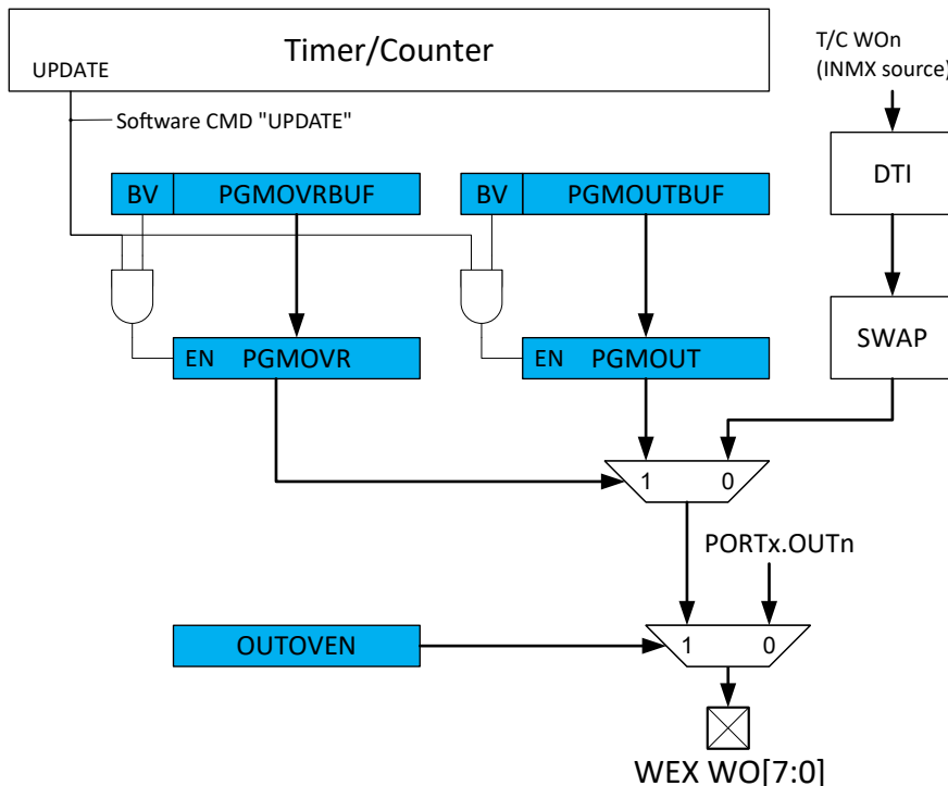
Figure 24-6. Pattern Generator Block Diagram
