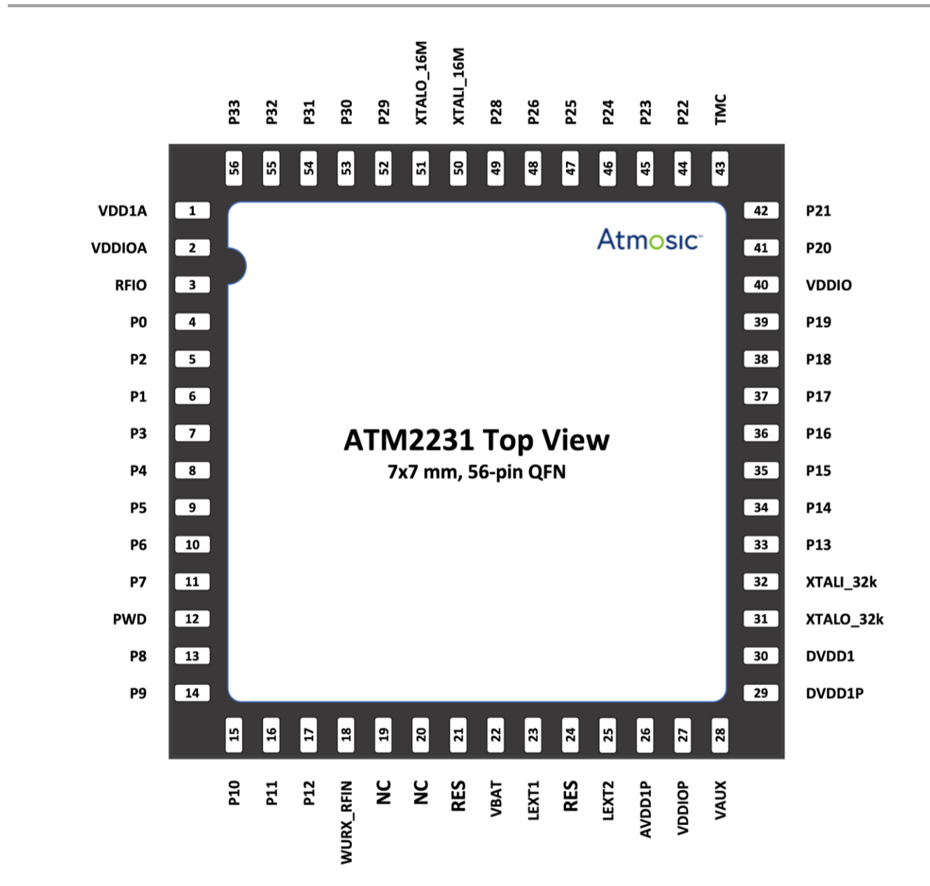
Figure 3.3-1 ATM2231 56-Pin 7x7 mm QFN Pinout (Top View)
