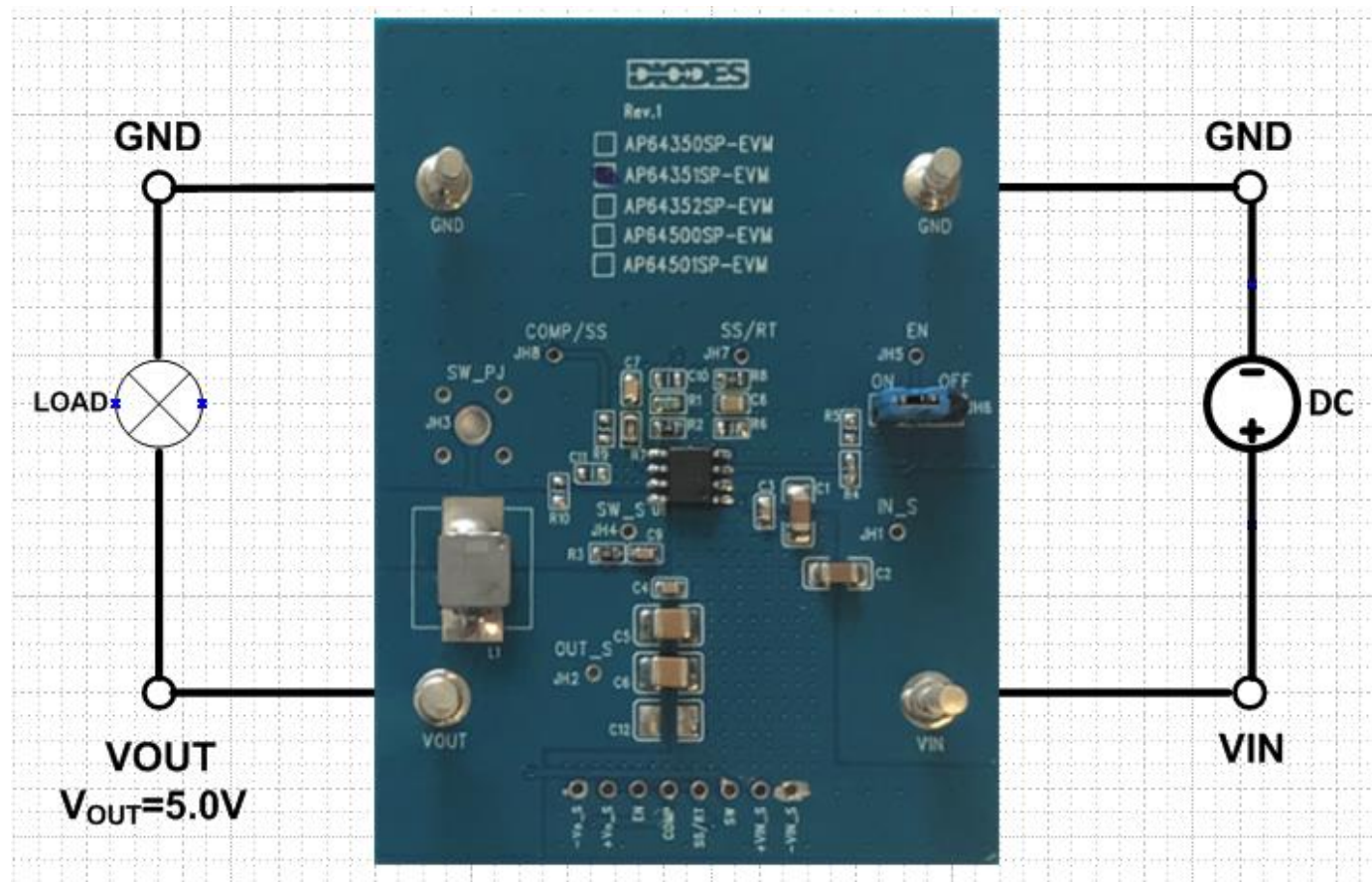
Figure 2. AP64351QSP-EVM
