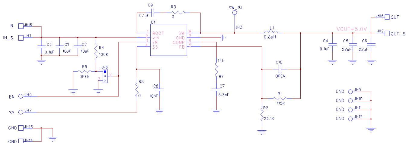
Figure 3. AP64351QSP-EVM Schematic
