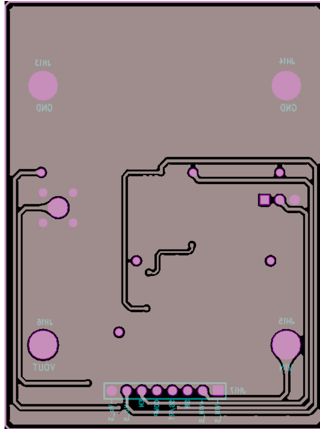
Figure 5. AP64351QSP-EVM – Bottom Layer
