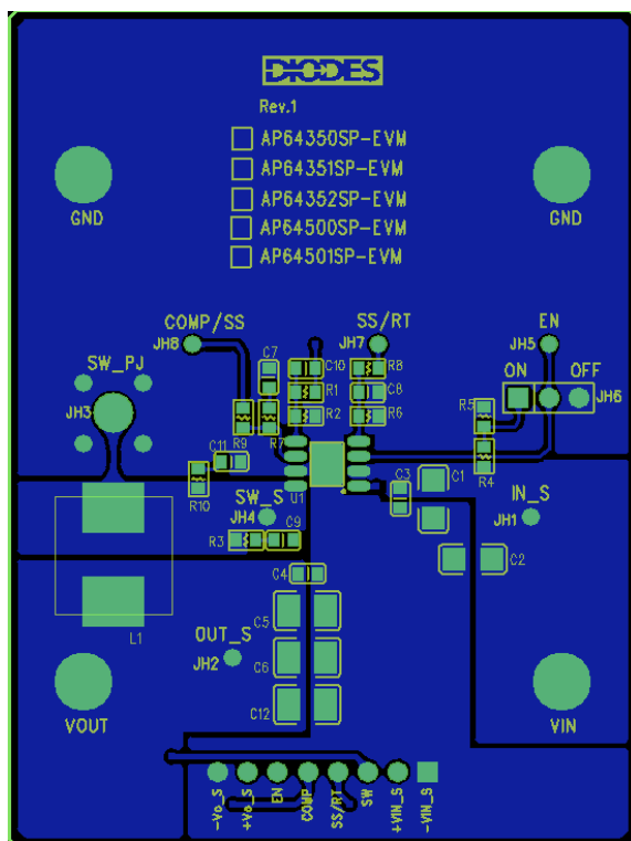
Figure 4. AP64351QSP-EVM – Top Layer
