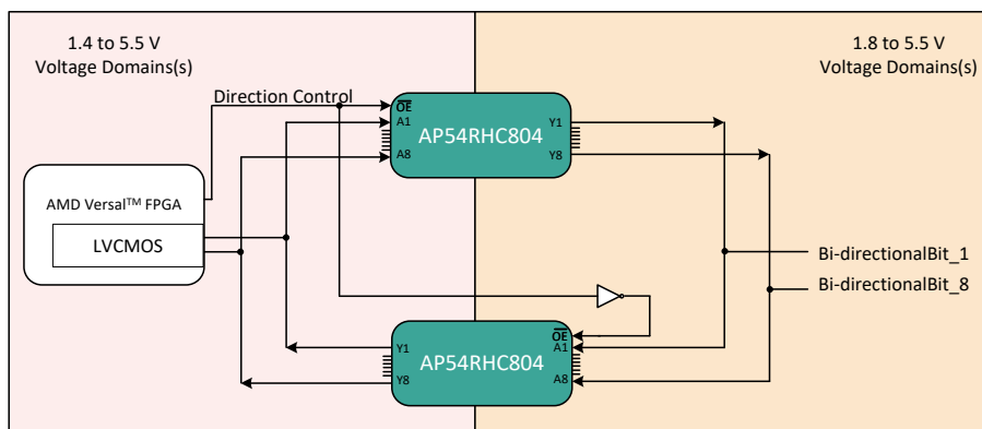
Figure 10: Bi-directional Level Shifting using Two AP54RHC804 Devices
