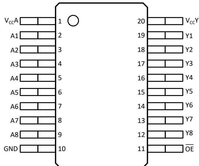
Figure 2: AP54RHC804 Device Pinout
