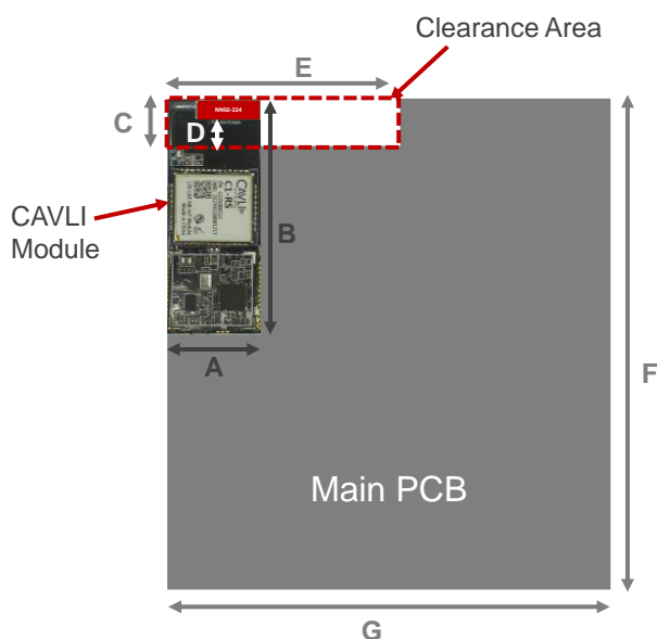
Figure 7 – P32 C1-RS module integrated in a main board for providing operation from 824MHz to 960MHz, and from 1710MHz to 1880MHz.
