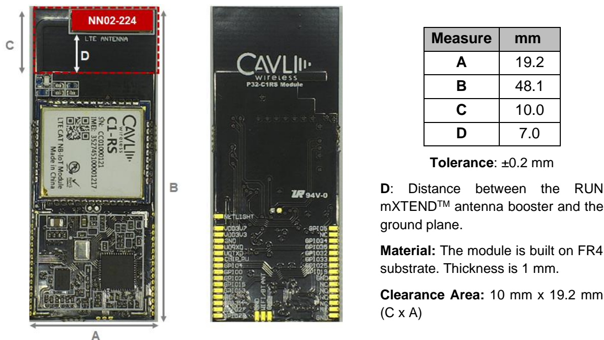
Figure 3 – P32 C1-RS Module integrates the RUN mXTEND ™ , providing operation from 824MHz to 960MHz, and from 1710MHz to 1880MHz. Top view in the left and bottom view in the right.
