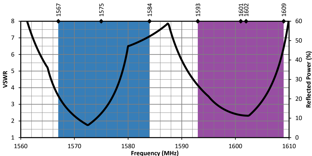
Figure 2. GNSSCP-SM12L1 VSWR
