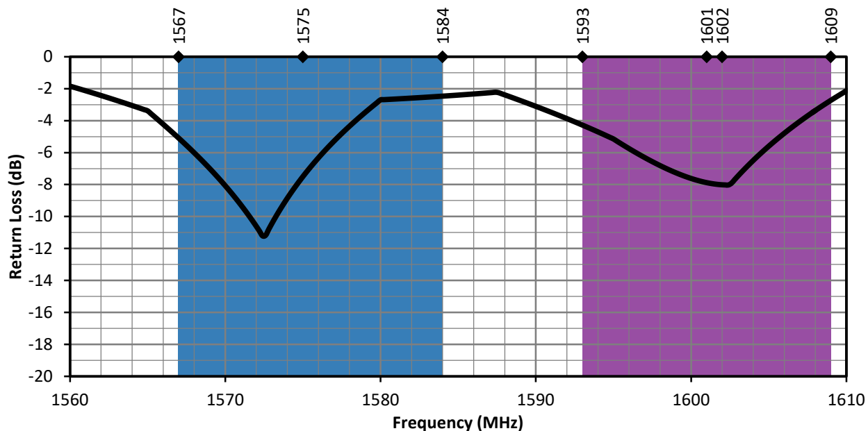
Figure 3. GNSSCP-SM12L1 Return Loss
