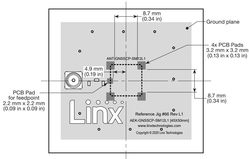
Figure 11. ANT-GNSSCP-SM12L1 Antenna Placement on PCB
