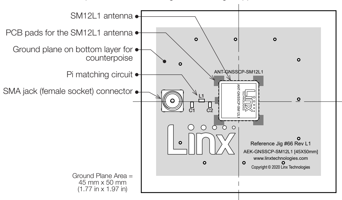
Figure 9. GNSSCP-SM12L1 Recommended Layout
