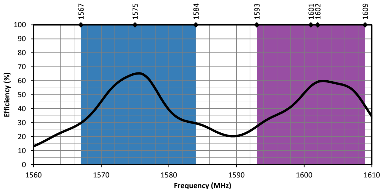
Figure 7. GNSSCP-SM12L1 Antenna Radiation Efficiency
