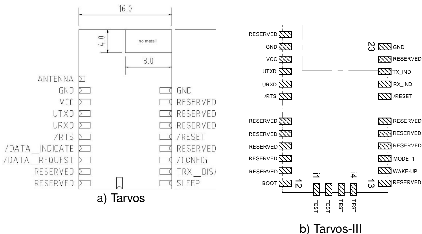
Figure 4: Pinout
