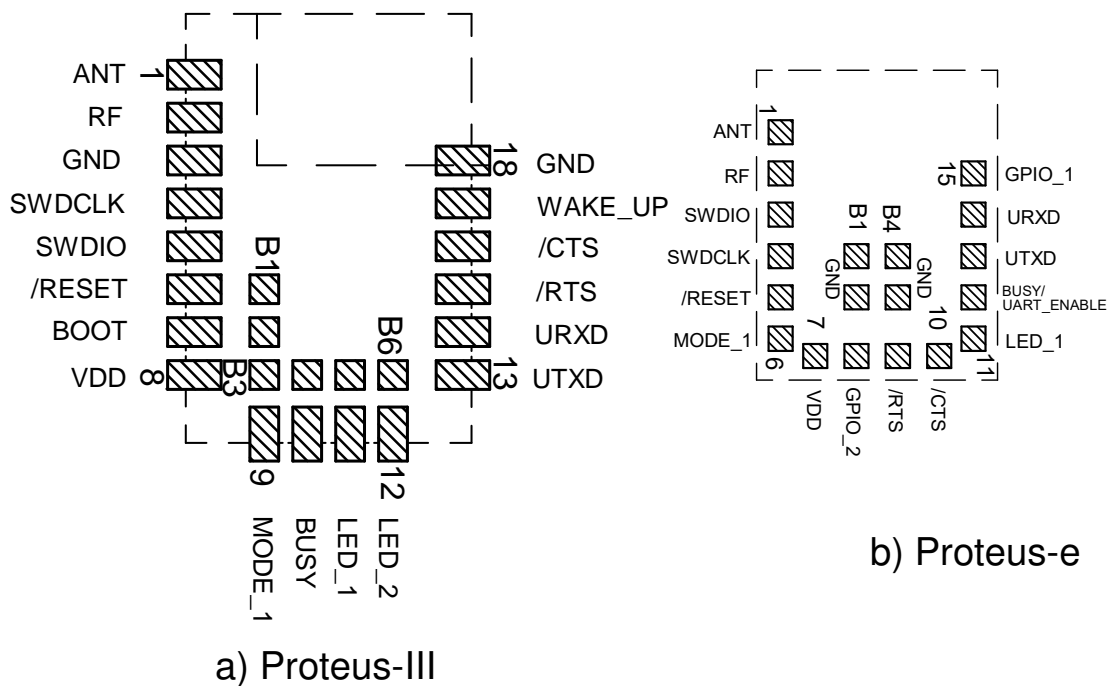
Figure 19: Pinout
