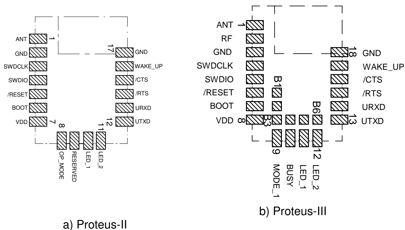
Figure 15: Pinout
