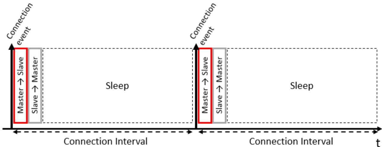
Figure 1: Data transmission with 1 packet per connection interval
