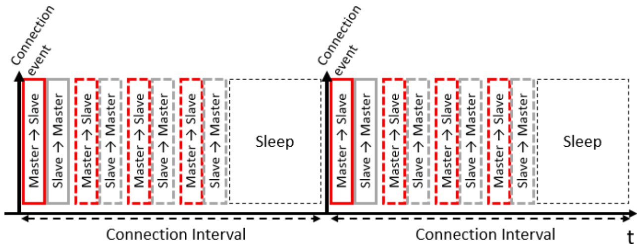
Figure 2: Improved data transmission with up to 4 packets per connection interval
