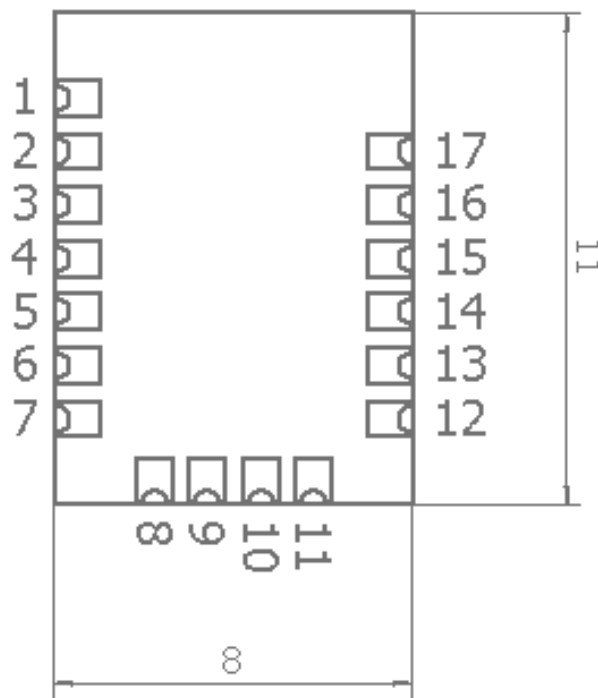
Figure 5: Pinout
