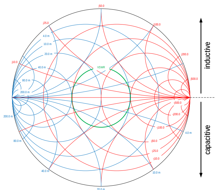
Figure 8: Example of a Smith Chart with conductance and susceptance lines (blue), and resistance and reactance lines (red). Additionally, this Smith Chart includes a VSWR circle (green)
