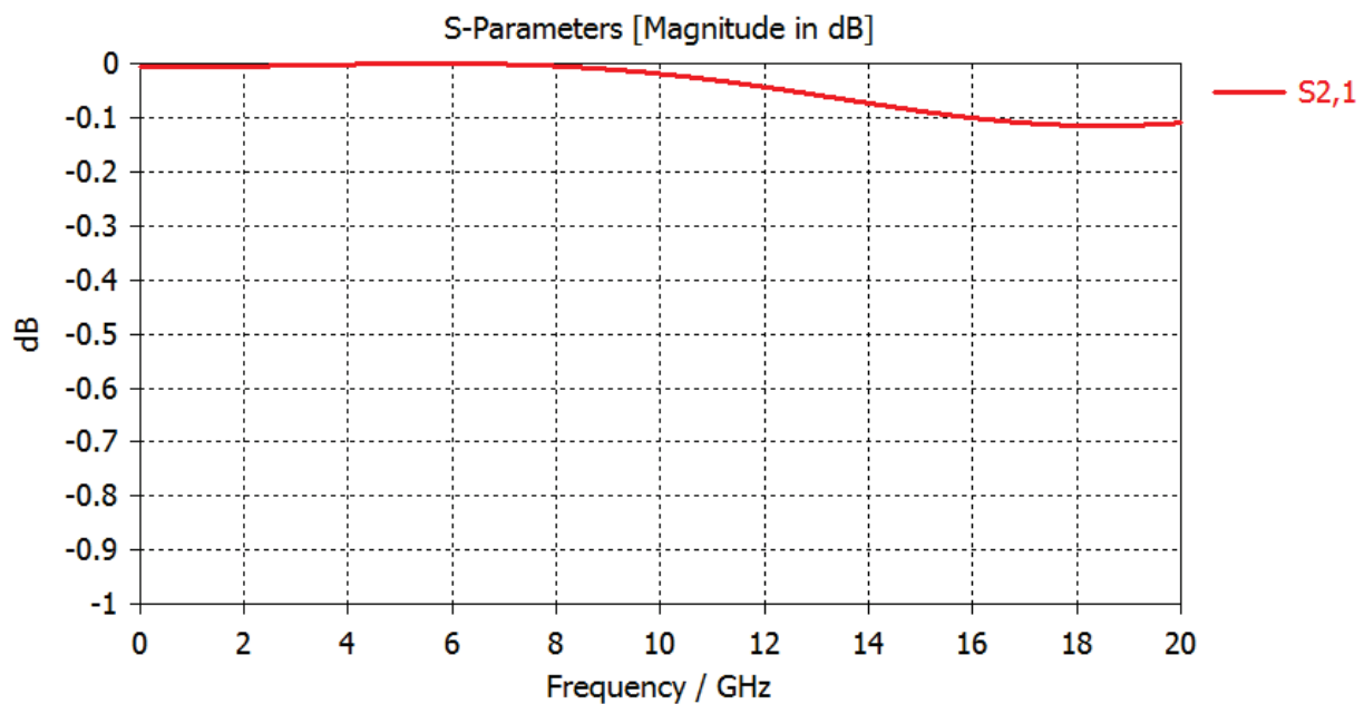
Figure 37: Result of S-Parameter – Return Loss measurement (Matching Design)
