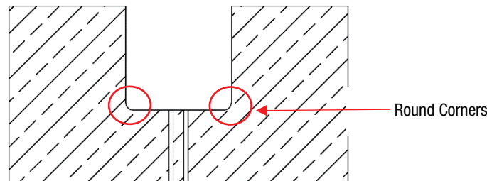
Figure 26: Round corners cause poor mechanical matching of the connector
