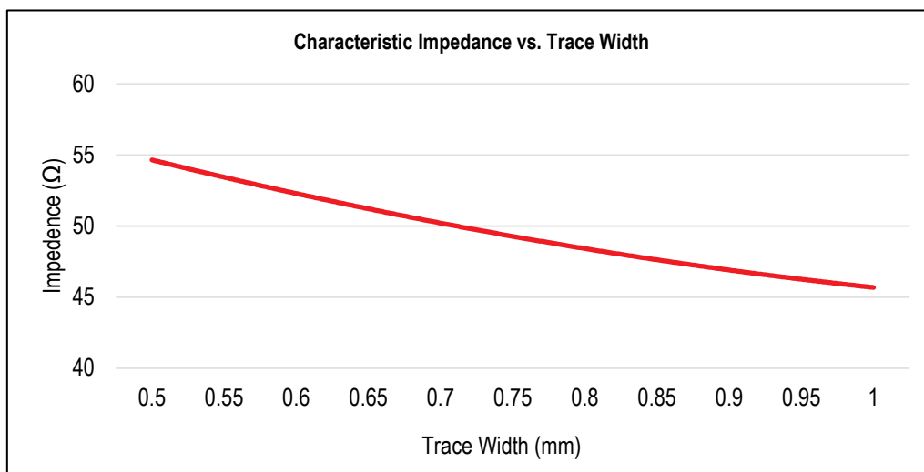
Figure 6: This figure shows impedance ( Z_0 ) is roughly inverse-proportional to trace width
