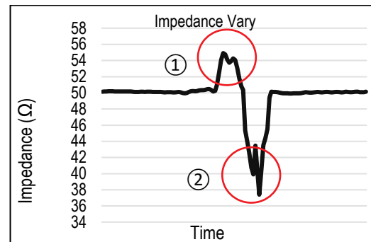
Figure 18: Impedance in time domain
