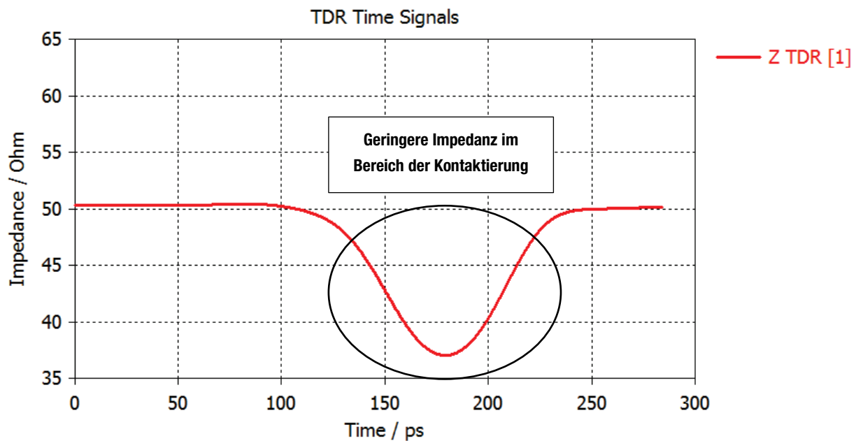
Figure 32: Result of TDR measurement (Original Design)
