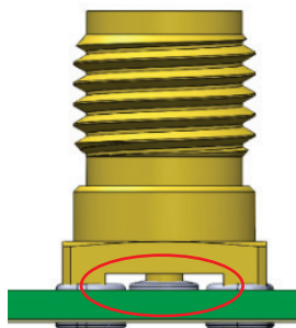
Figure 16: Gap between PCB and connector
