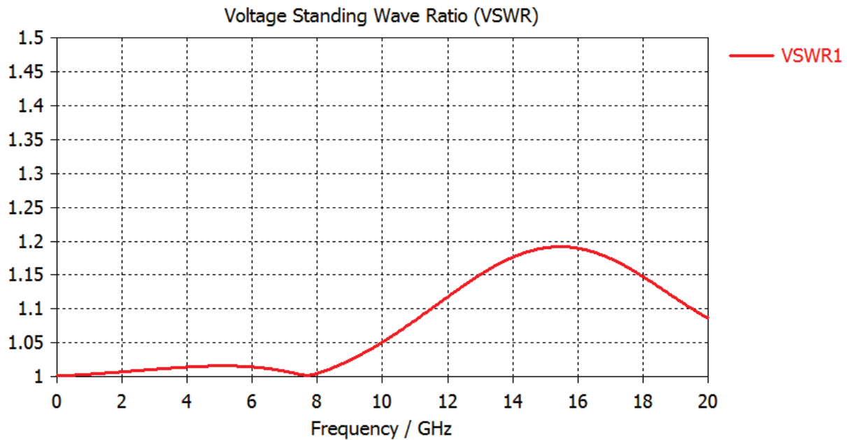
Figure 36: Result of S-Parameter - VSWR measurement (Matching Design)
