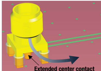
Figure 17: Signal route: Connector interface PCB trace
