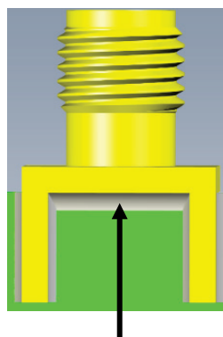
Figure 28: Use solder paste to fill up the gap
