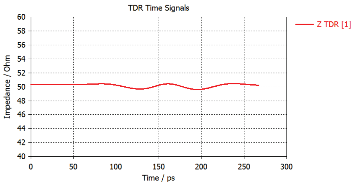
Figure 33: Result of TDR measurement (Matching-Design)
