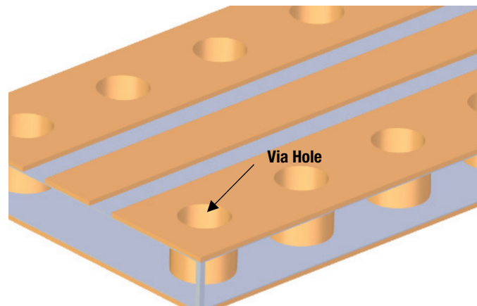
Figure 29: Via implementation from the coplanar ground traces to the ground (GND) layer
