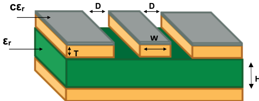
Figure 4: Coplanar waveguide
