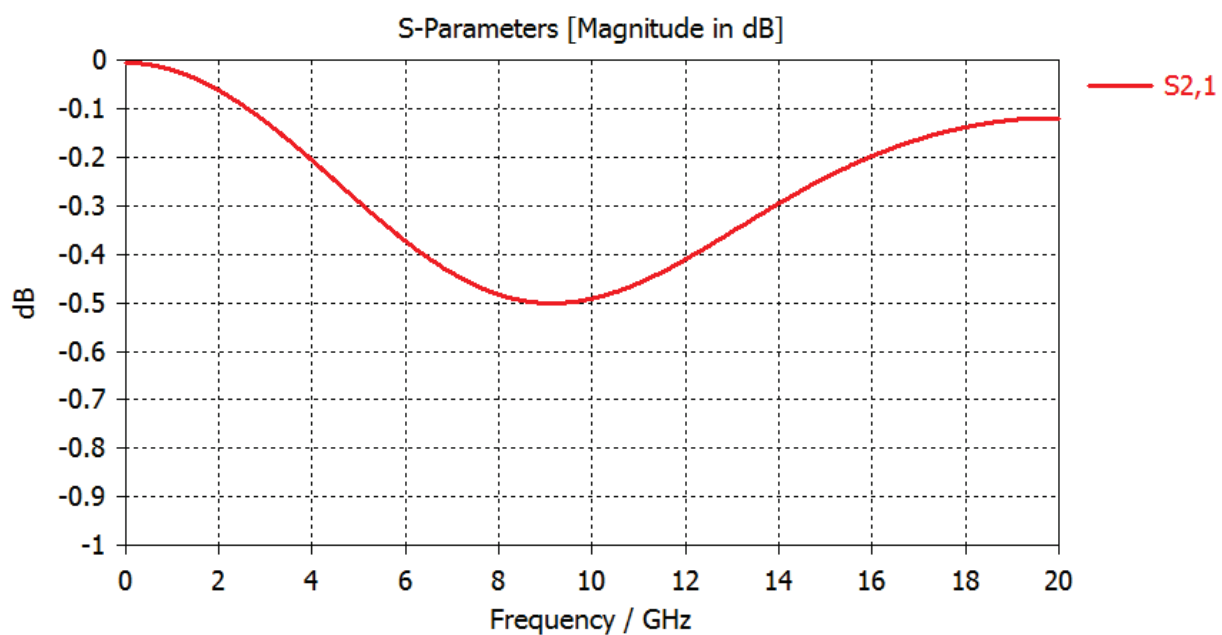
Figure 35: Result of S-Parameter - Return Loss measurement (Original Design)
