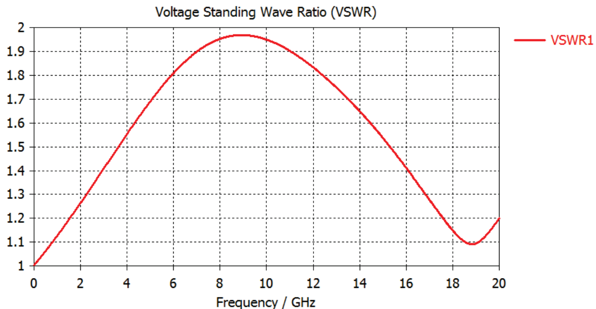
Figure 34: Result of S-Parameter – VSWR measurement (Original Design)
