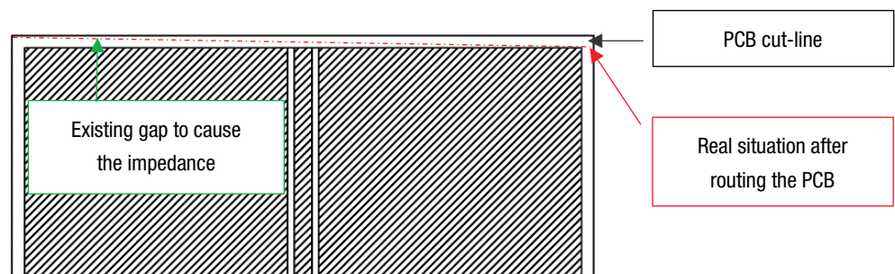
Figure 23: Ground not extended to end of the PCB
