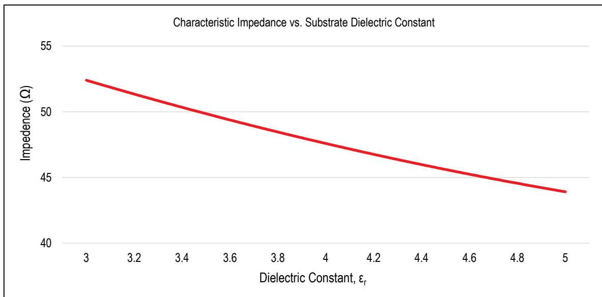
Figure 5: This figure shows impedance (Z 0 ) is inversely proportional to dielectric constant (ε r )
