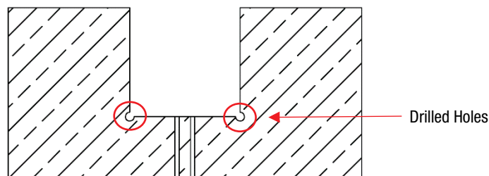
Figure 27: Additional relief holes improve the fit of the connector
