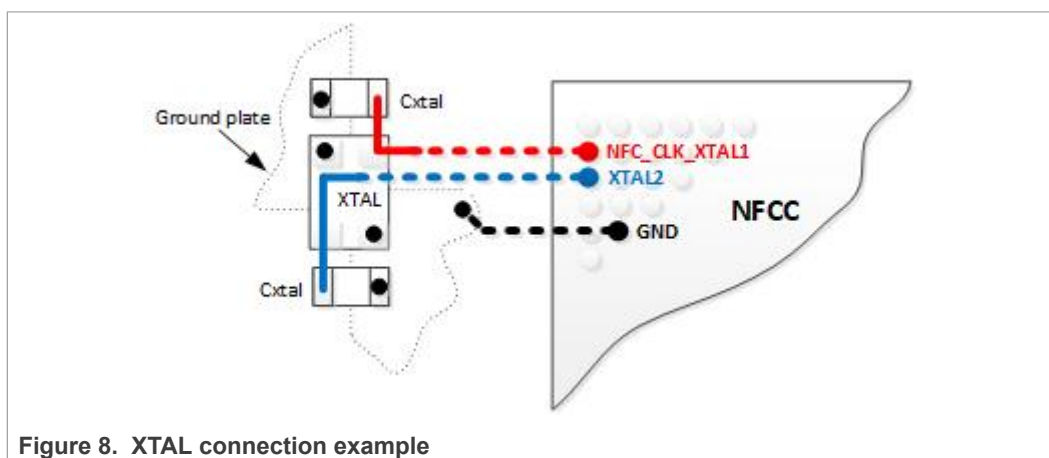
Figure 8. XTAL connection example
