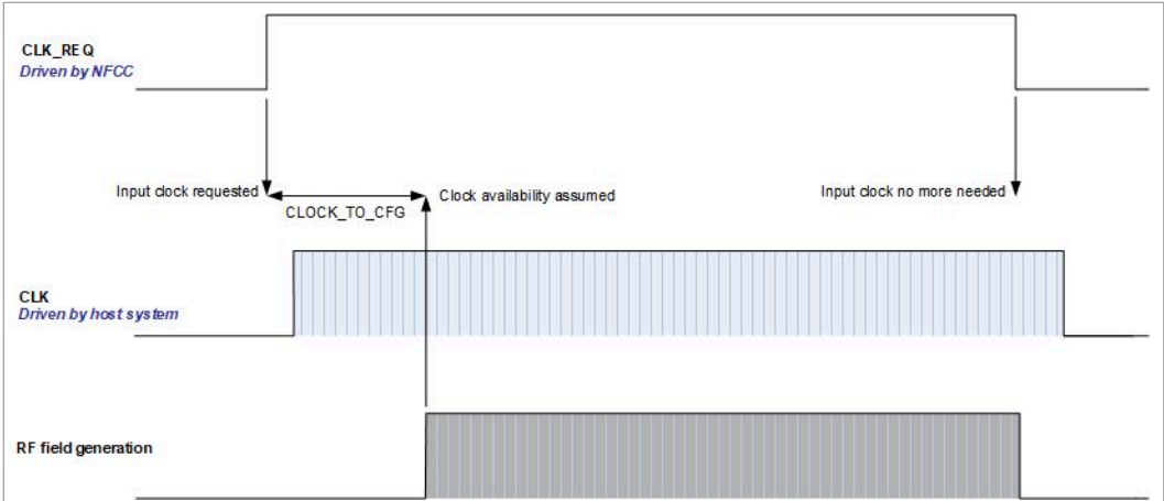
Figure 11. Clock request through CLK_REQ pin
