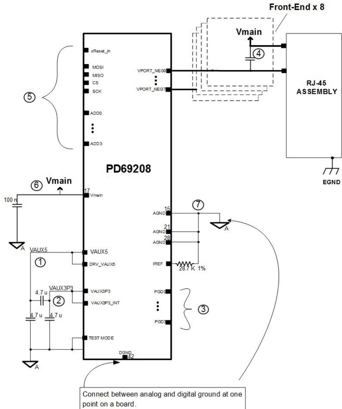
Figure 30 • Component Identification for PD69208 Circuitry
