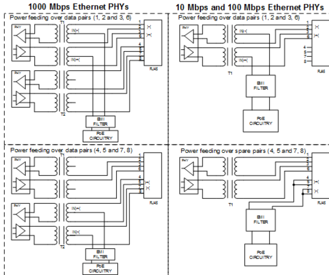
Figure 29 • Output Ports Design Details
