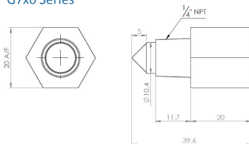
Figure 3-5 Product Dimensions – Optomax Industrial Glass Range
