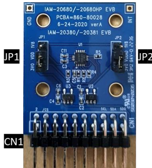
Figure 3. EVB jumpers and connectors
