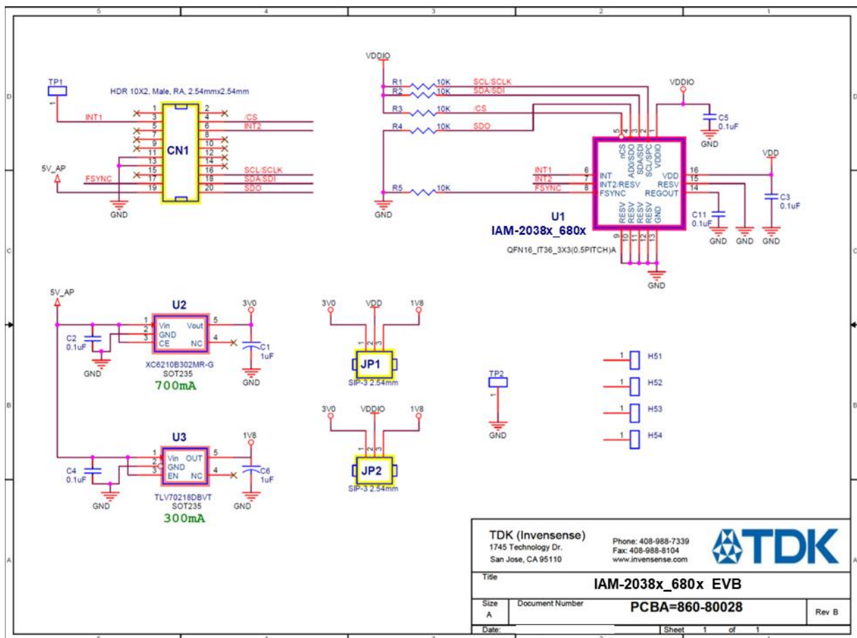
Figure 2. EVB circuit schematic
