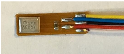
Figure 7. EV_ICS-41350-FX Top View
