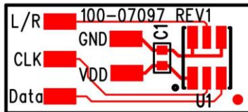
Figure 4. EV_ICS-41351-FX Board Layout (Top View)
