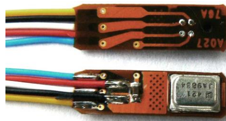
Figure 8. Bottom Port Mic Top and Bottom View (All Others)
