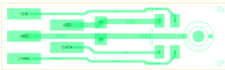
Figure 2. EV_ICS-41350-FX Board Layout (Top View)
