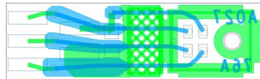
Figure 3. Bottom Port Mic Evaluation Board Layout (Top View)
