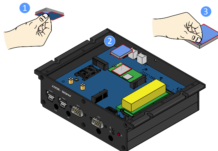
Figure 28: Installing the M.2 SATA SSD thermal pad
