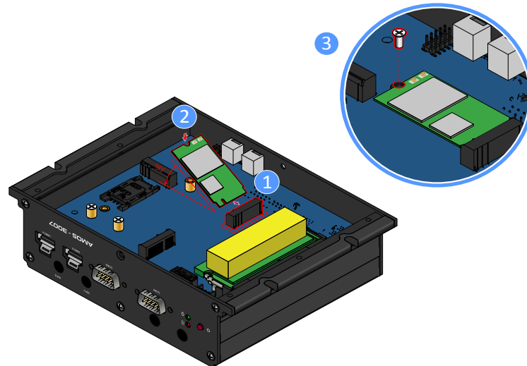
Figure 27: Inserting the M.2 SATA SSD module
