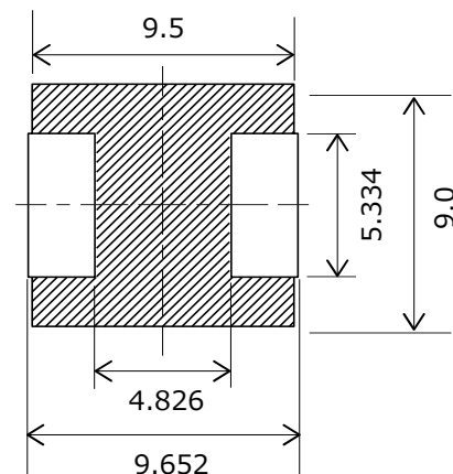
Series PCC-M0840M-LP (ETQP4M□□□KVK)
