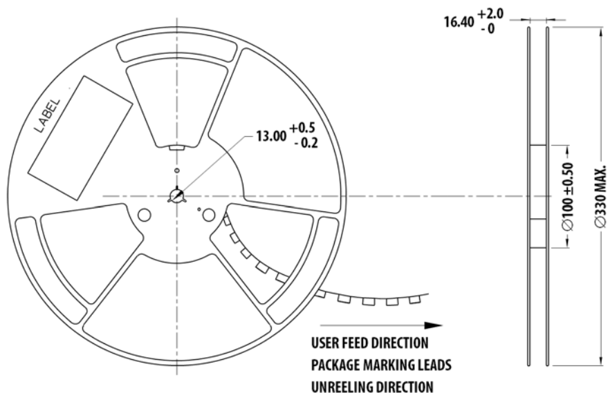
Figure 12: Reel Dimensions
