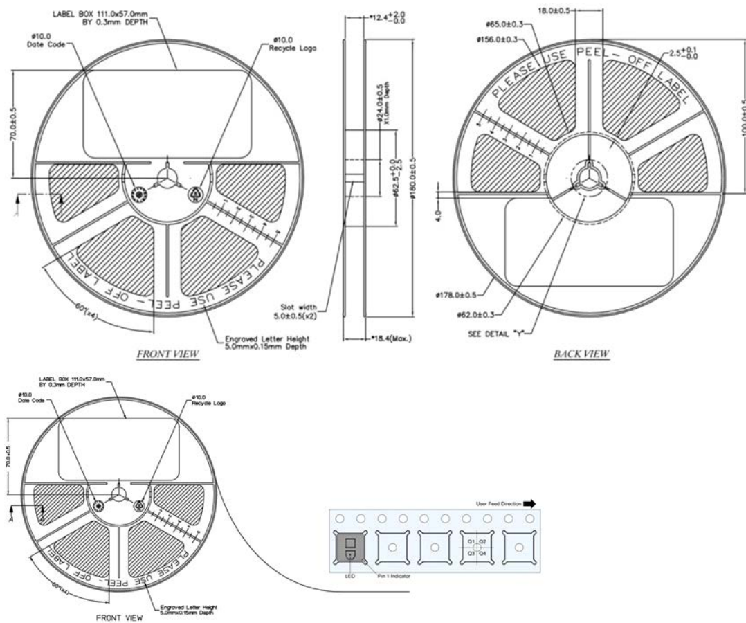
Figure 12: AEDR-9930E2 Reel Dimensions and Orientation
