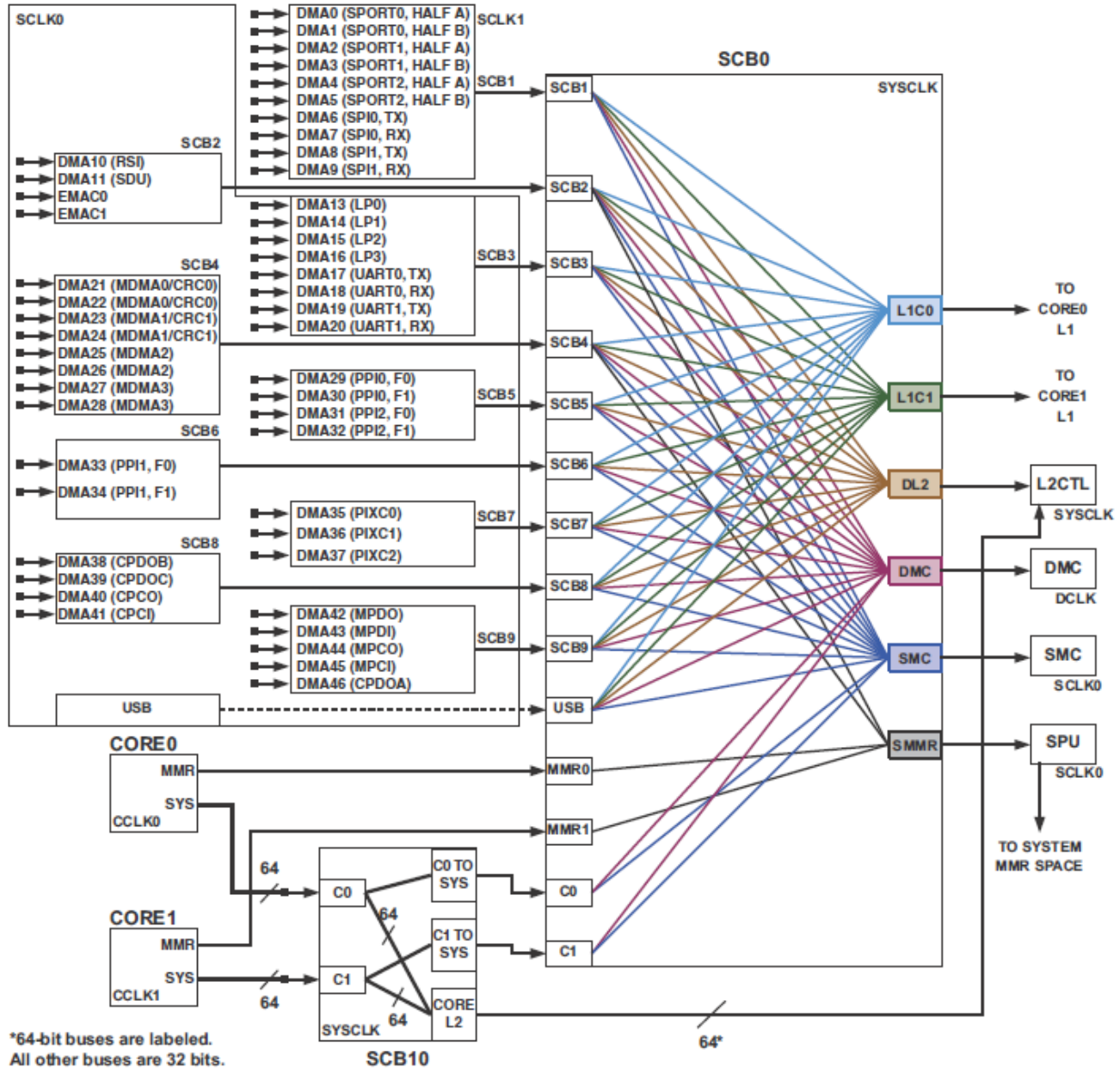
Figure 1. ADSP-BF609 Processors system architecture
