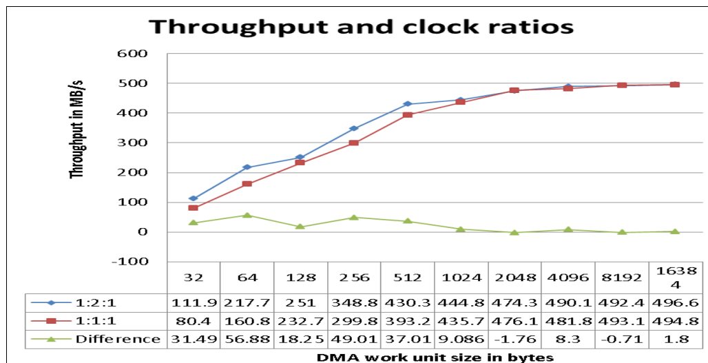
Figure 5. DMC throughput comparison for different clock ratios
