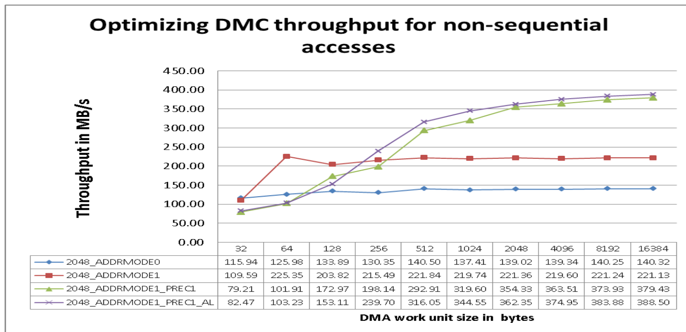
Figure 10. Optimizing throughput for non-sequential accesses
