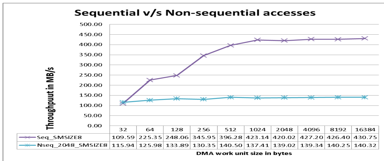
Figure 9. DMC throughput for non-sequential read accesses compared with sequential accesses
