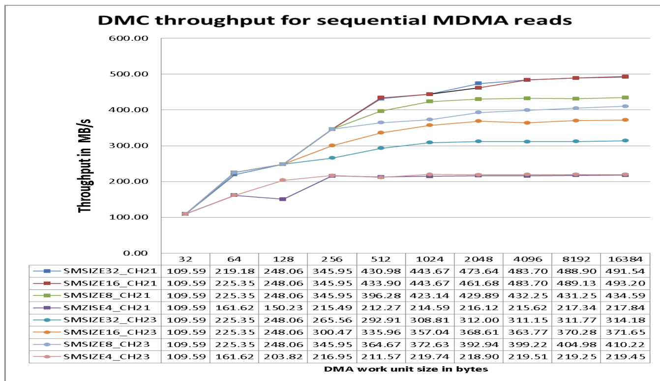
Figure 7. DMC measured throughput for sequential MDMA reads
