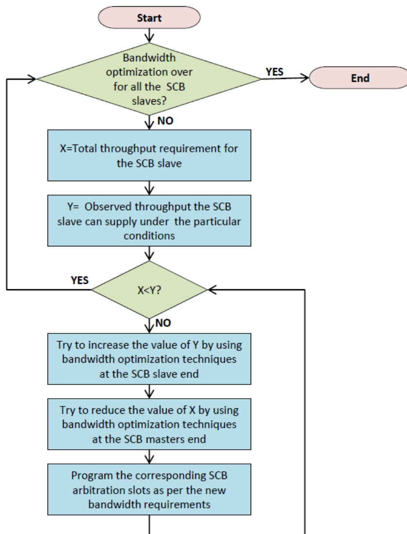
Figure 14. Typical system bandwidth optimization procedure
