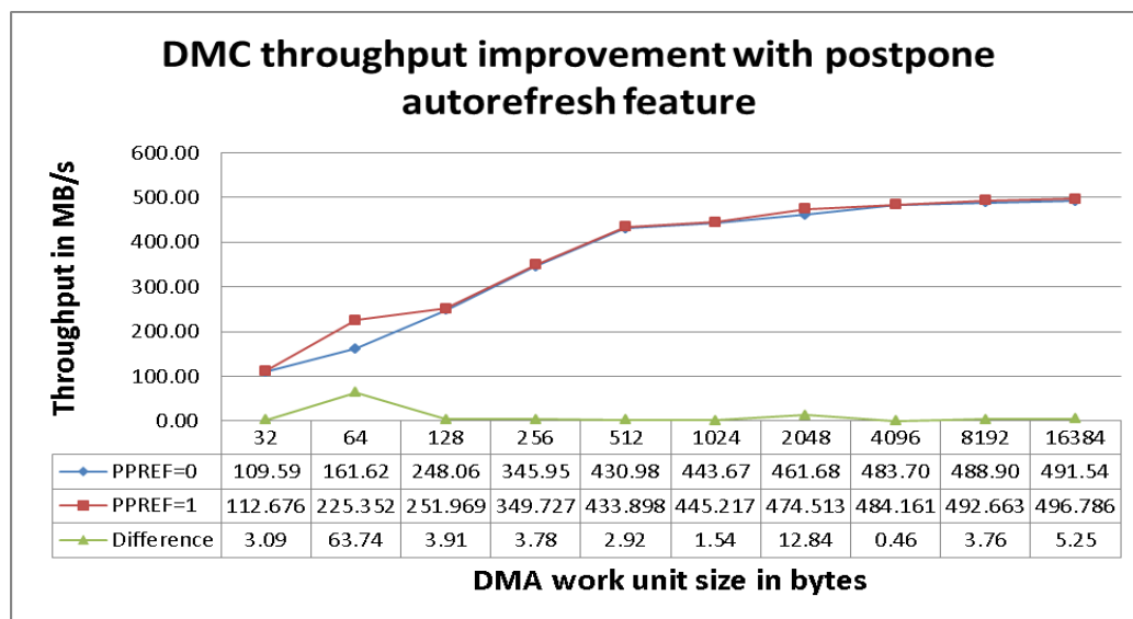
Figure 13. DMC throughput optimization with Postpone Autorefresh feature
