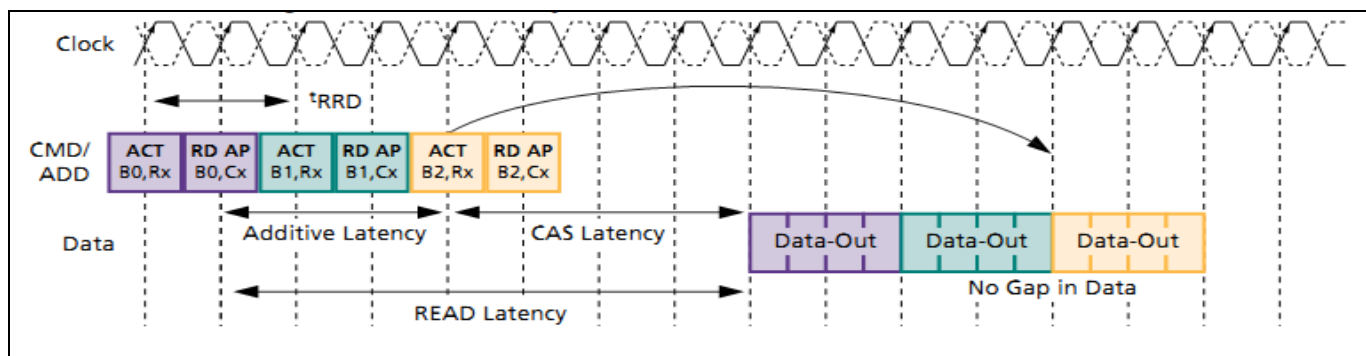
Figure 12. DDR2 reads with additive latency
