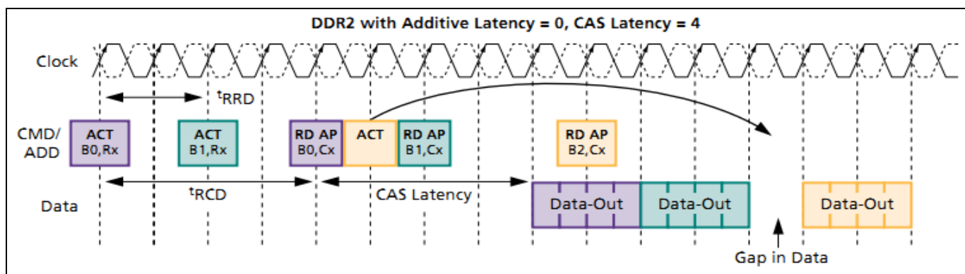
Figure 11. DDR2 reads without additive latency
