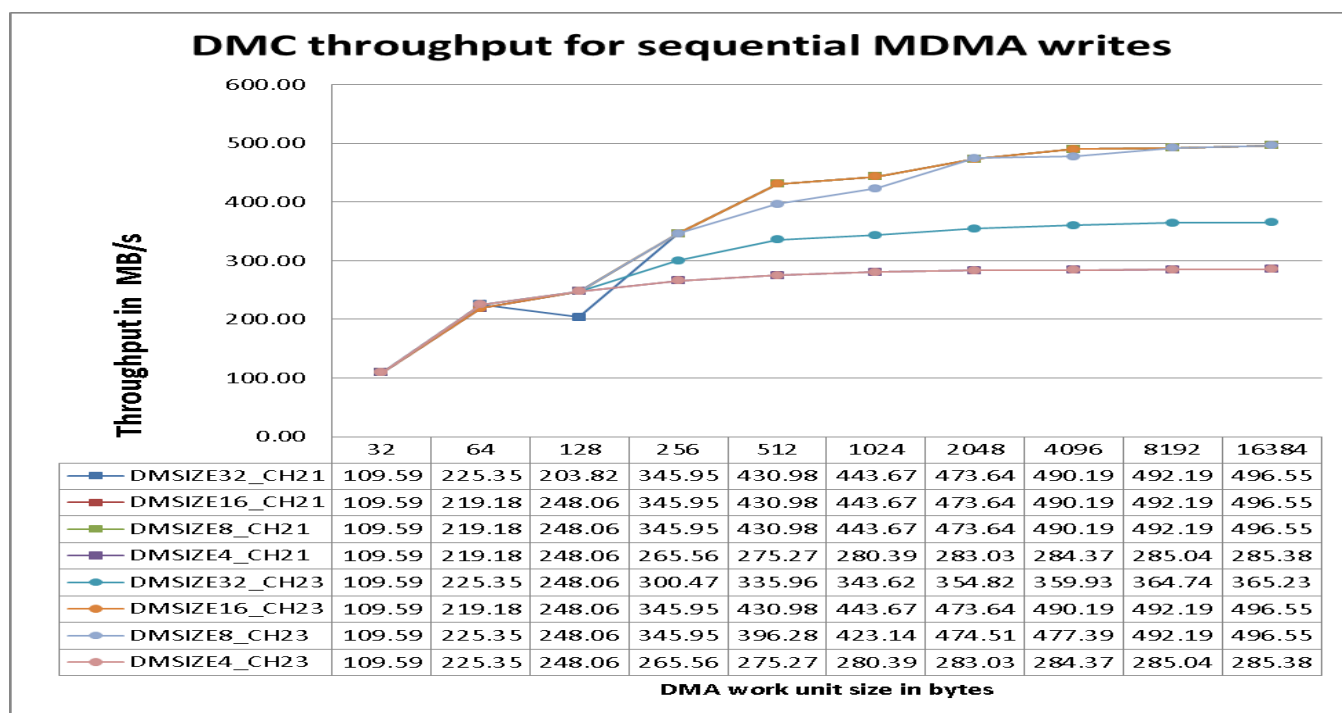
Figure 8. DMC measured throughput for sequential MDMA writes
