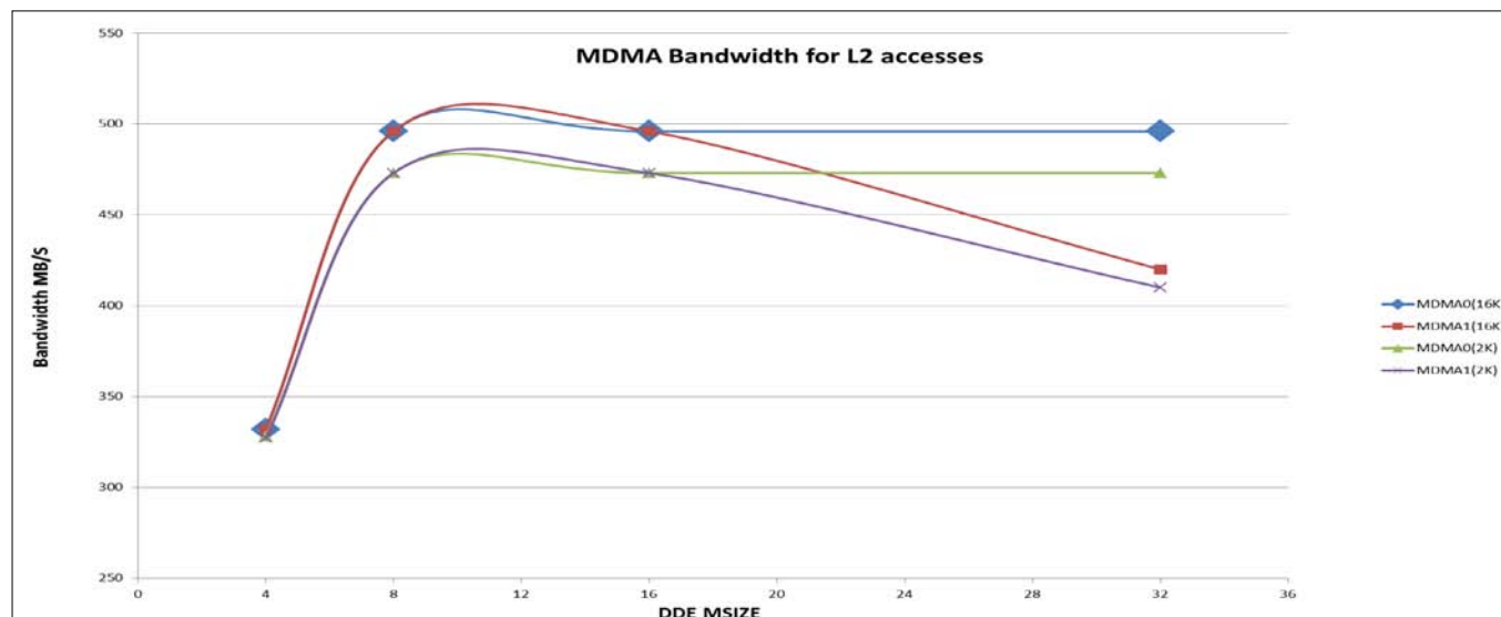
Figure 6. L2 MDMA read throughput for different MSIZE and work unit size values
