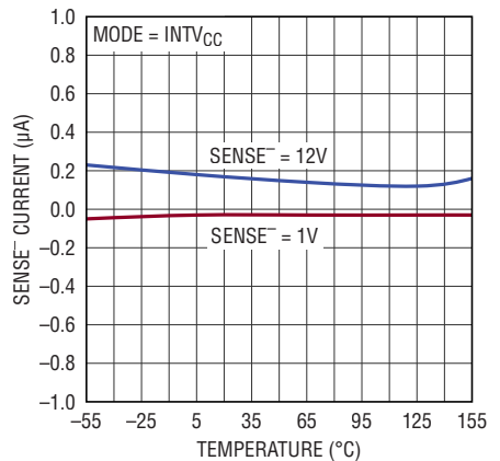
SENSE1,2 - Current vs Temperature
