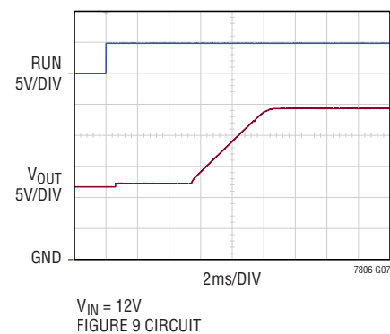
Soft Start-Up
