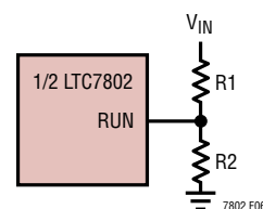
Figure 5. Using the RUN Pins As a UVLD
