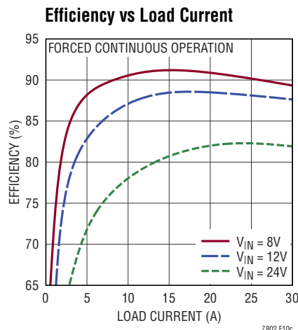
Figure 10. 2.25MHz 2-Phase Single Output 3.3V, 24A Step-Down Regulator
