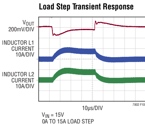
Figure 10. 2.25MHz 2-Phase Single Output 3.3V, 24A Step-Down Regulator
