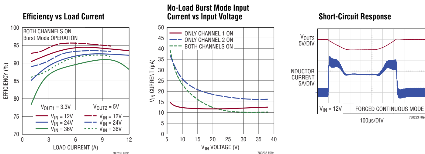
Figure 9. High Efficiency Dual 3.3V, 5V Step-Down Regulator with Spread Spectrum
