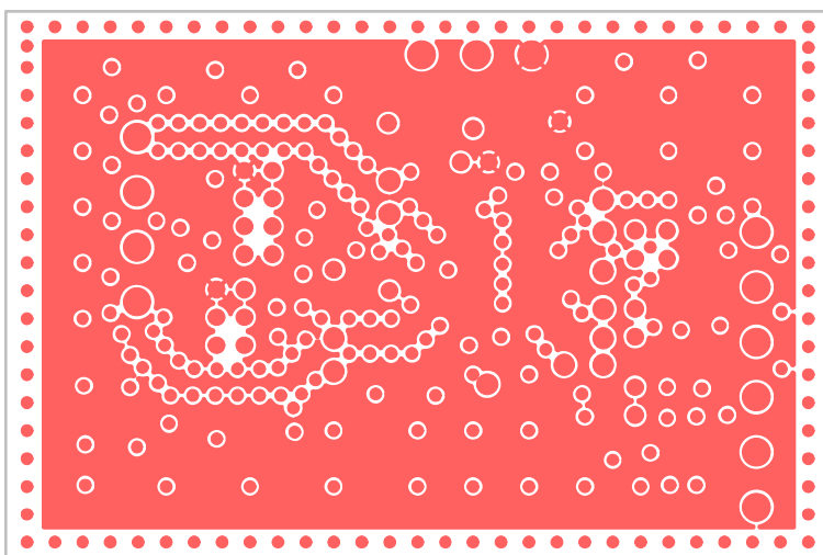
Figure 7. EVAL-ADM3064EEBZ, Layer 3
