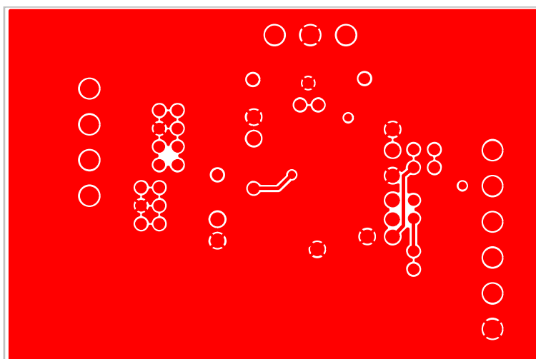
Figure 8. EVAL-ADM3064EEBZ, Layer 4
