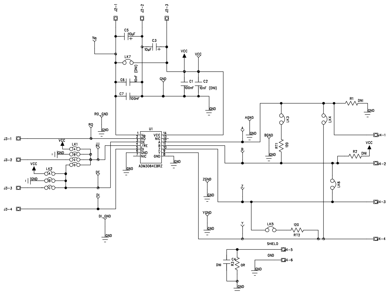
Figure 4. EVAL-ADM3064EEBZ Schematic
