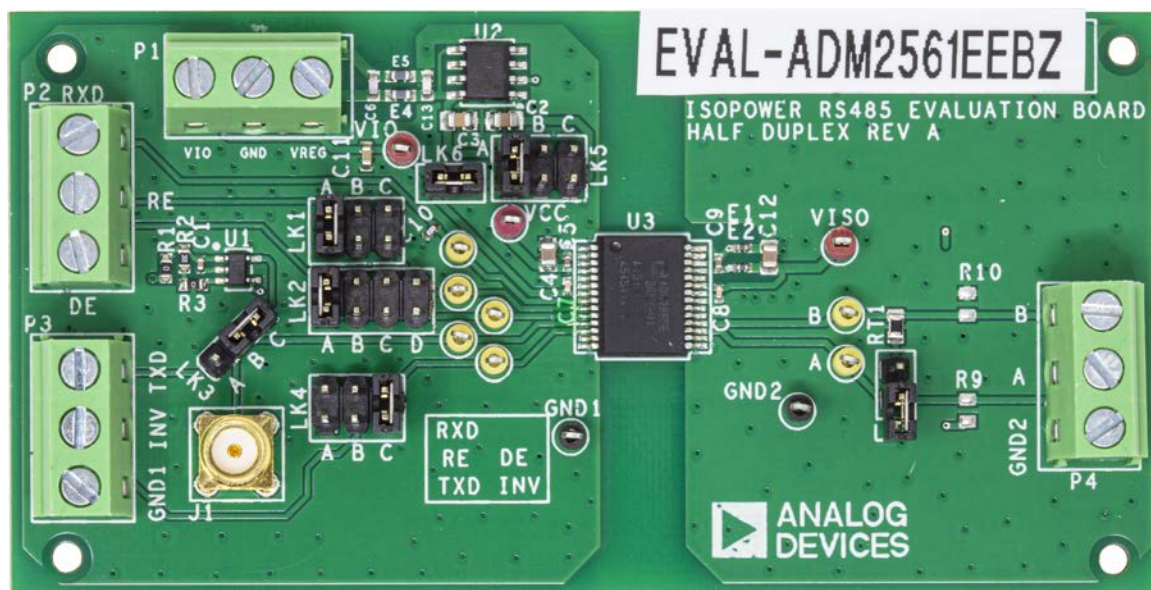
Figure 1. EVAL-ADM2561EEBZ
