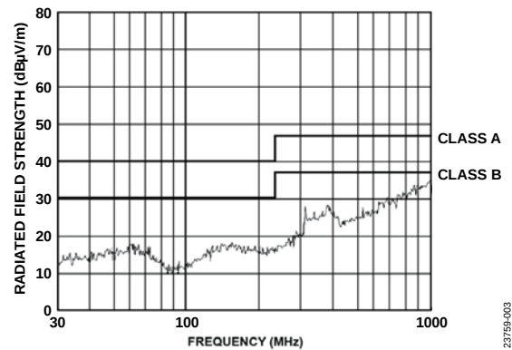
Figure 4. CISPR 32/EN 55032 Radiated Emissions Results
