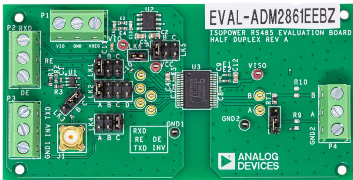
Figure 2. EVAL-ADM2861EEBZ
