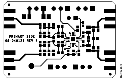
Figure 4. ADA4945-1CP-EBZ Evaluation Board Layout Pattern, Primary Side
