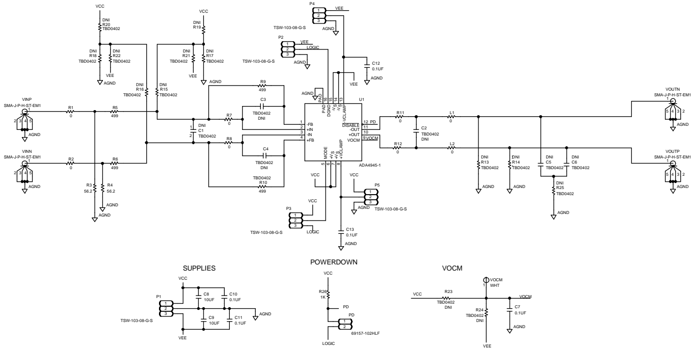
Figure 2. ADA4945-1CP-EBZ Evaluation Board Schematic
