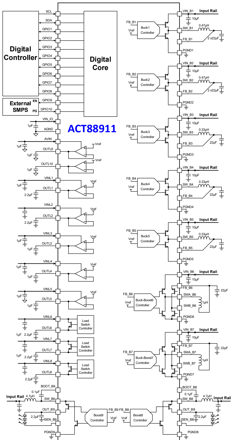
Figure 3: ACT88911 Block Diagram & Application Schematic (Buck-Boost 6/7 in Buck Mode)
