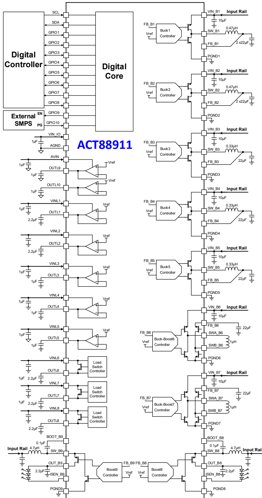
Figure 2: ACT88911 Block Diagram & Application Schematic (Buck-Boost 6/7 in Buck-Boost Mode)
