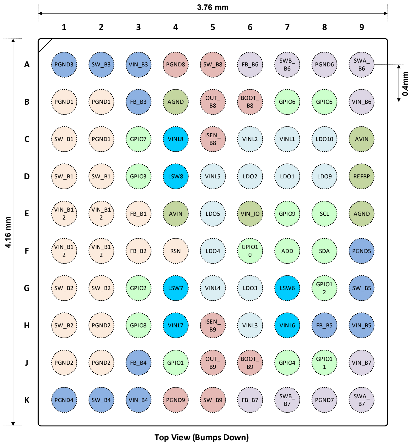
Figure 4: ACT88911 Pin Configuration – Top View (bumps down) – WLCSP- 90
