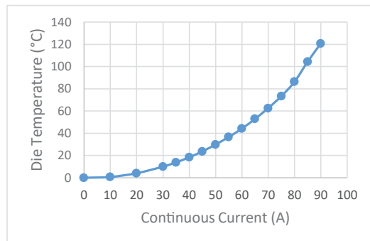
Figure 19: Self-heating in the MC package due to current flow
